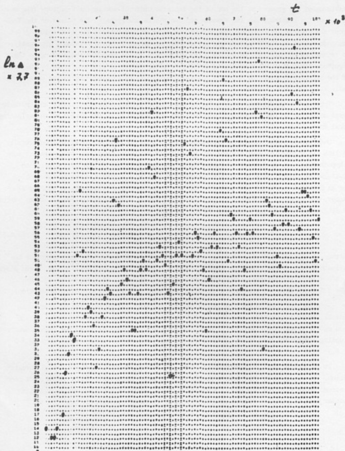
Fig. 3.6.14: The same as Fig. 3.6.13, except that: \psi_{10} \approx 0.670 ; \psi_{20} \approx 0.640 ; the motion is stable.
