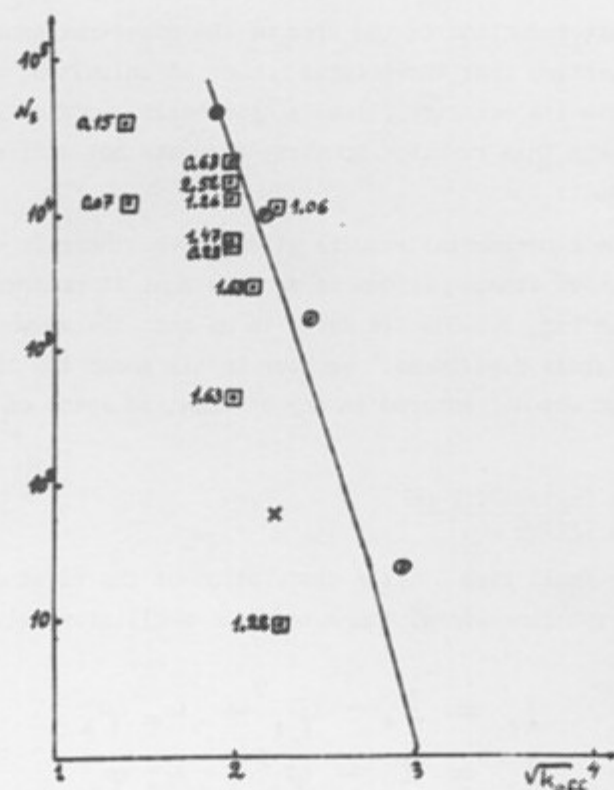
Fig. 3.5.4: The dependence of the number of stable bins of the phase plane ( N_s ) on the parameter k_{eff} for various cases: \odot - force (3.2.6); \gamma = 0.63 ; \times - force (3.2.5); \gamma = 0.74 ; \square - force (3.2.3) and (3.2.4); the values of \gamma are indicated near the dots; the continuous line is an analytical estimate according to formula (3.5.1).
