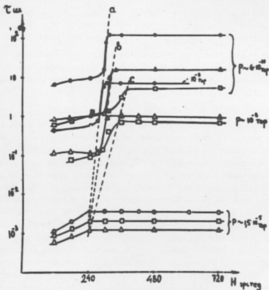
Fig. 4.4.1. Dependence of the lifetime of electrons in a magnetic mirror trap on the strength of the magnetic field H .
