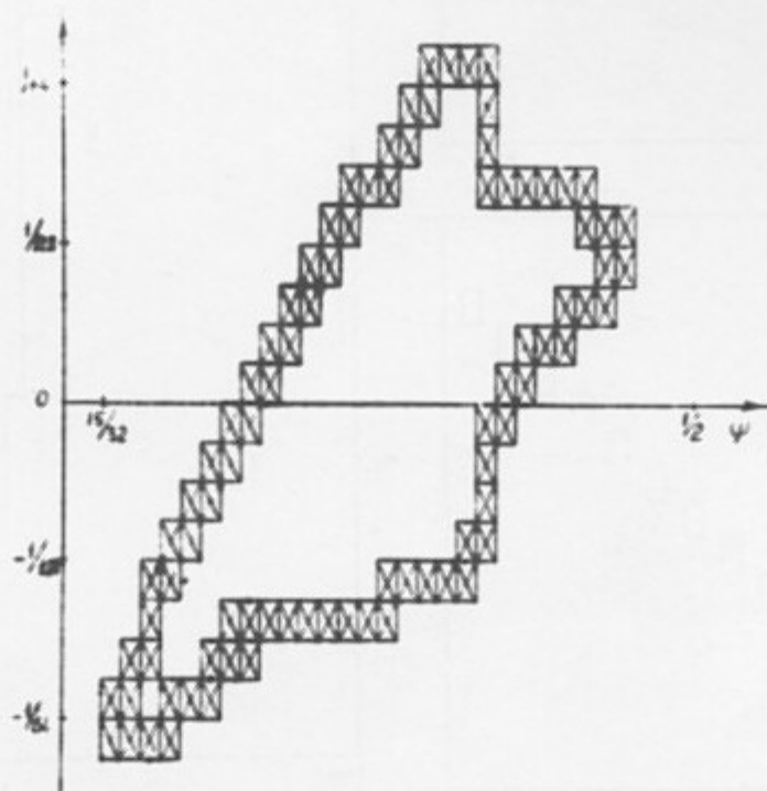
Fig. 3.5.1: An "islet" of stability for a special value of k = 60.1993377 ; \psi_0 = 0.01 ; \psi_0 \approx 0.483 ; t = 10^8 ; size of bin (1/512) \times (1/1024) ; the picture does not contradict the ideally thin curve corresponding to an absolutely stable trajectory.
