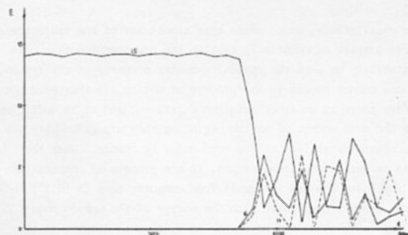
Fig. 4.6.2 Excitation of single (15th) mode: E_{15} \approx 14.1 ; \beta \approx 0.0314 ; c \approx 0.04 ; t_{\max} = 9000 ; h = 1/6 ; \Delta E/E \approx 1.5\% .
