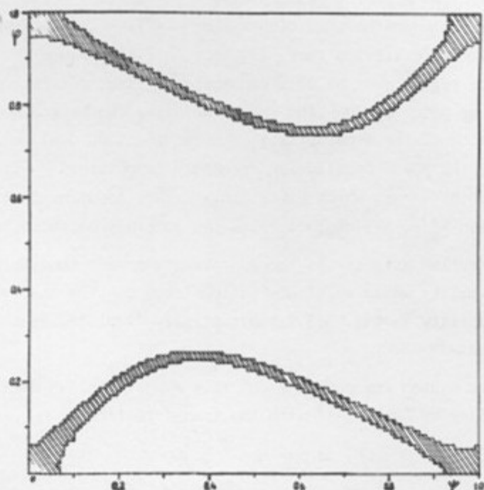
Fig. 3.3.5: Phase map for the analytical "force" (3.2.6): 128 \times 128 bins; k \approx 0.62 ; t = 10^7 . The hatched region represents the stochastic layer in the vicinity of the separatrix of the main resonance.
