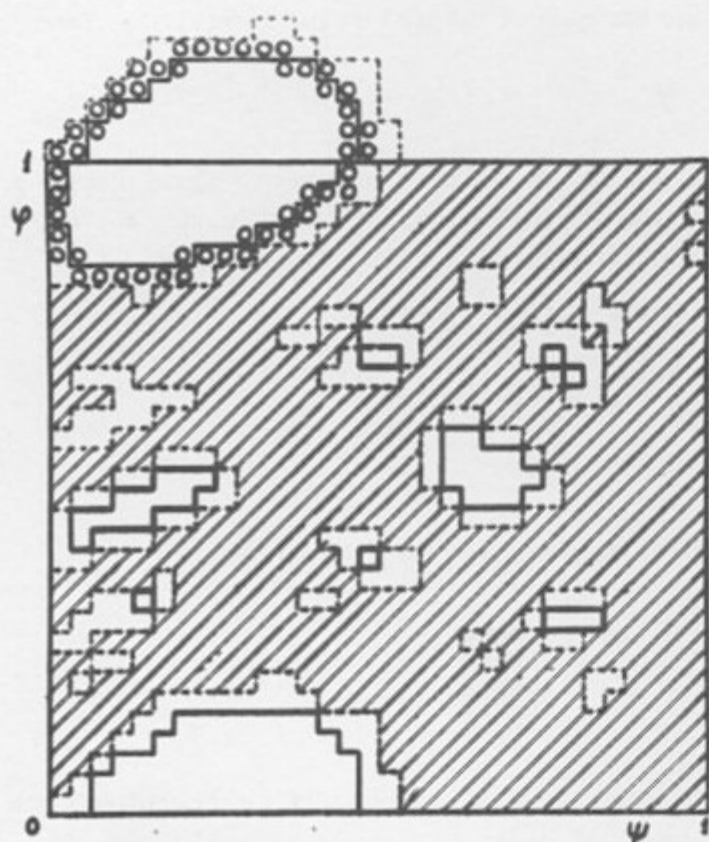
Fig. 3.3.1: Phase map of system (3.2.1) for "force" (3.2.5); divided into 32 \times 32 bins: k \approx 1 ; \psi_0 = 0 ; \phi_0 \approx 0.765 ; t = 5 \times 10^6 steps; the stochastic region is hatched; the bins completely free from the trajectory are shown by an unbroken line; between the unbroken and dotted lines are bins with considerably less density of trajectory (only part of the bin occupied by the stochastic component); the small circles represent the stable trajectory with initial conditions \psi_0 = 0 ; \phi_0 \approx 0.460 ; t = 5 \times 10^6 .
