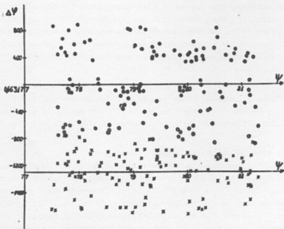
Fig. 3.3.8: Search for the correlation \Delta\psi, \psi : ○ - the beginning of the long computation; × - the end of the long computation (see Fig. 3.3.7).
