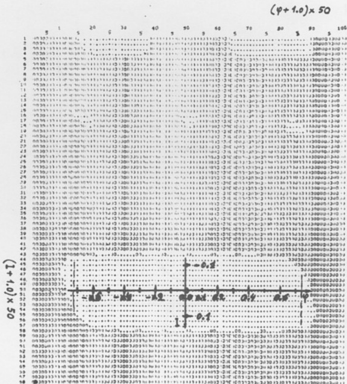
Fig. 3.6.1: The region of one-dimensional stability for model (3.6.1); \mu_0 = 0 ; t = 10^5 .
