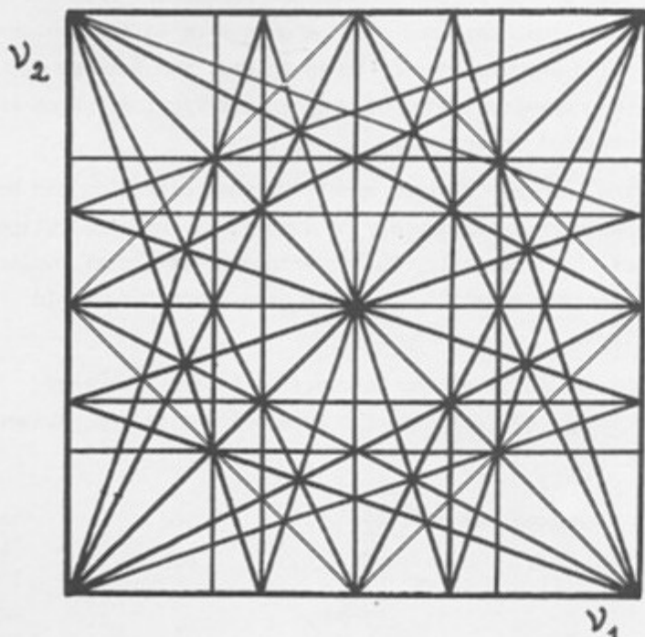
Fig. 4.3.1. Set of resonances n_1 \nu_1 + n_2 \nu_2 + p \nu_0 = 0 for \nu_0 = 1 ; |n_1| + |n_2| \leq 4 ; p is any integer; 40 different resonances in all.
