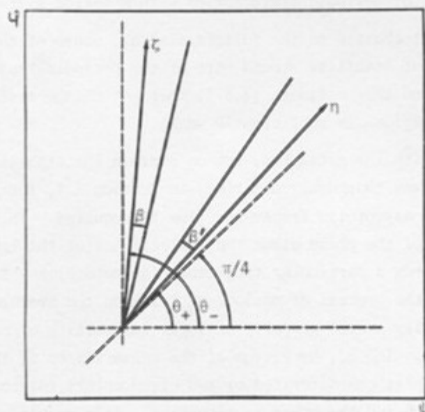
Fig. 2.8.1: Structure of transversal transformation for elementary model (2.8.1) in the absence of stable regions (2.8.3): \theta_{\pm} indicate the direction of extension and contraction eigenvectors; \beta, \beta' represent the border between contraction and extension cones (sectors) before and after transformation, respectively.
