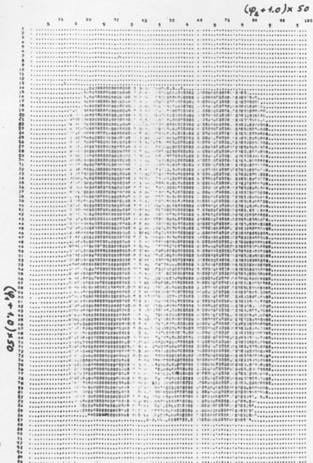
Fig. 3.6.3: Phase map of the case in Fig. 3.6.2 near the beginning of the computation: t = 10^7 . The circles mark the bins occupied by the trajectory and the dots give the coordinate network.
