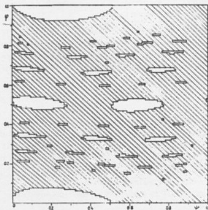
Fig. 3.3.2: The phase map for "force" (3.2.5): 128 \times 128 bins; k = 0.2 ; t = 5 \times 10^7 ; the stochastic component is hatched.
