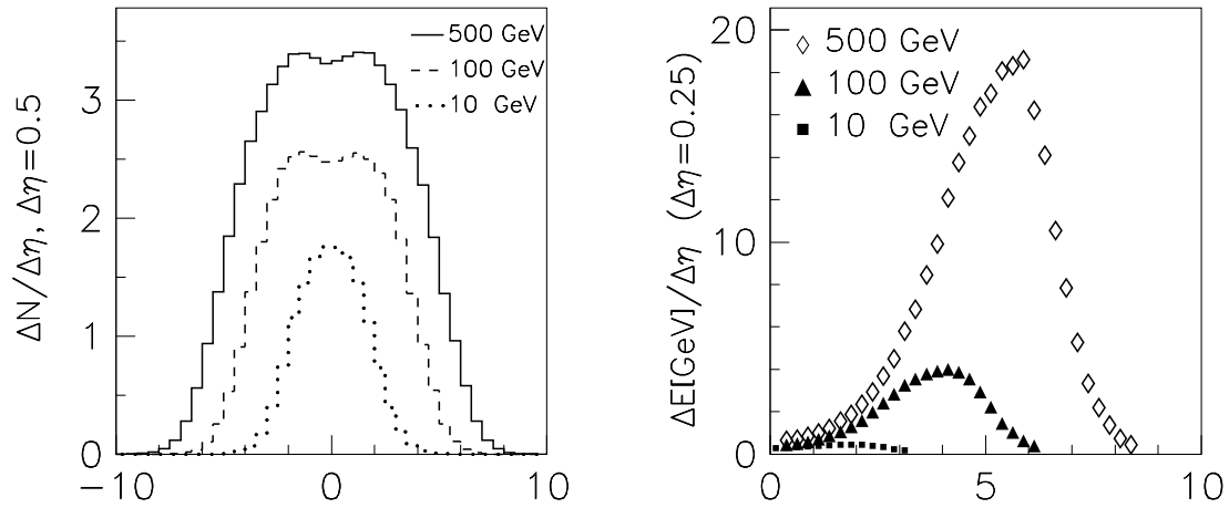
Figure A.16: Distribution of particle \eta (left) and energy flow (right) on pseudorapidity \eta in \gamma\gamma \rightarrow \text{hadrons} events (photons have equal energies).
