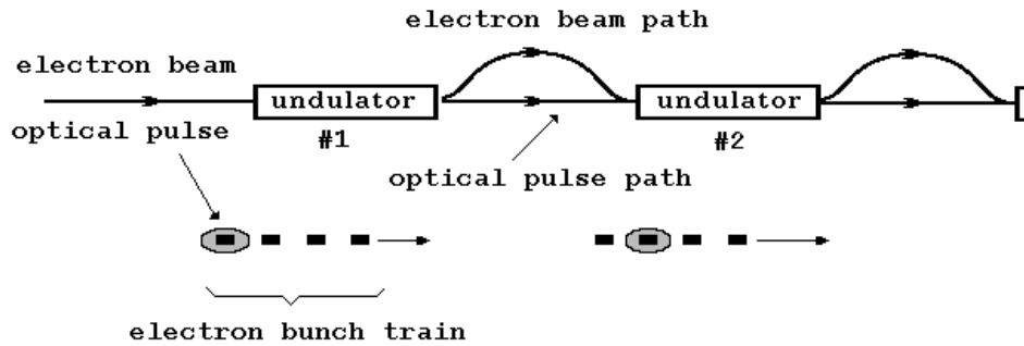
Figure A.26: The scheme of multi-stage FEL amplifier. One optical pulse is amplified by a sequence of electron bunches. The peak power of the output radiation exceeds by a factor of N (number of amplification stages) the peak output radiation power of traditional single pass FEL amplifier.
