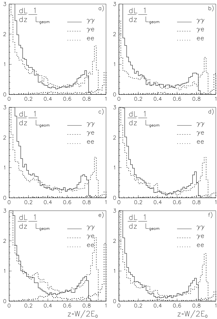
Figure A.10: Luminosity spectra for the scheme without deflection for the \gamma\gamma collider parameters presented in Tables A.2, A.3 (Figs. A.10a, b)... correspond to TESLA(1), TESLA(2)...). Luminosity distributions are normalized to the geometrical luminosity. For additional comments see the text.
