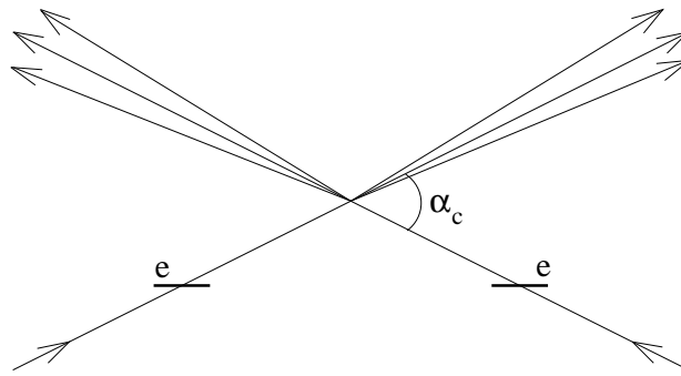
Figure A.9: Crab-crossing scheme.
