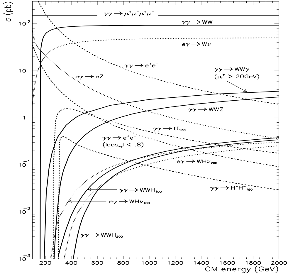
Figure A.2: The cross sections of some processes in \gamma\gamma and e\gamma collisions.
