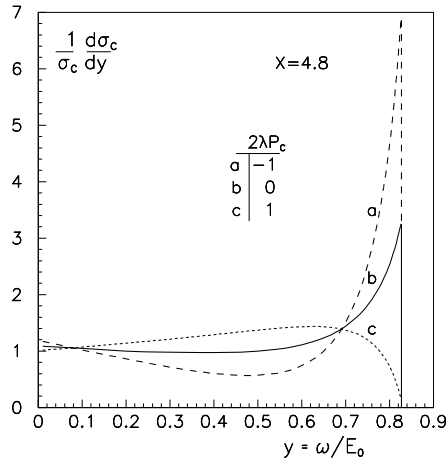
Figure A.4: Spectrum of the Compton scattered photons for different polarizations of the laser and electron beams.
