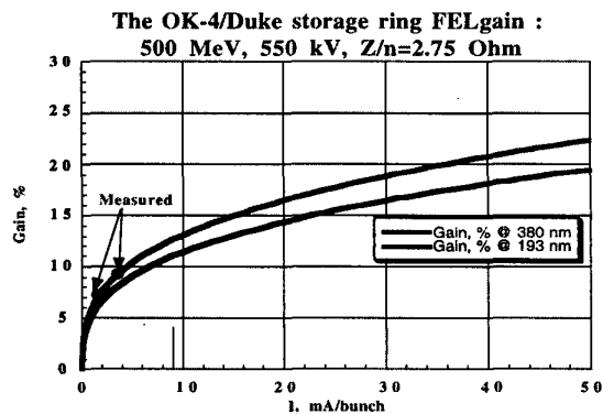
Fig. 2 The measured (dots, 345 nm) and predicted gain (solid lines) for 380 nm and 193 nm of the OK-4.
