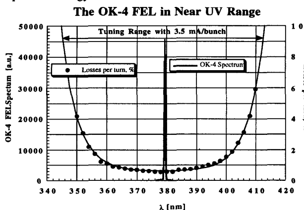
Fig. 1 The tuning range of the OK-4 FEL (with 3.5 mA/bunch at 500 MeV with 500 kV RF voltage) using 380 nm mirrors. The line in the center is a measured time lasing line. This line was tuned \pm 18\% from 345 to 413 nm by changing the current in the OK-4 wigglers. The dots are measured round trip cavity losses and the smooth curve is a fit. Round-trip losses at the edges of the tuning range give the value of the FEL gain at a given current: gain >9\% at 345 nm with 3.5 mA/bunch, 500 MeV electron beam and 500 kV RF voltage.
