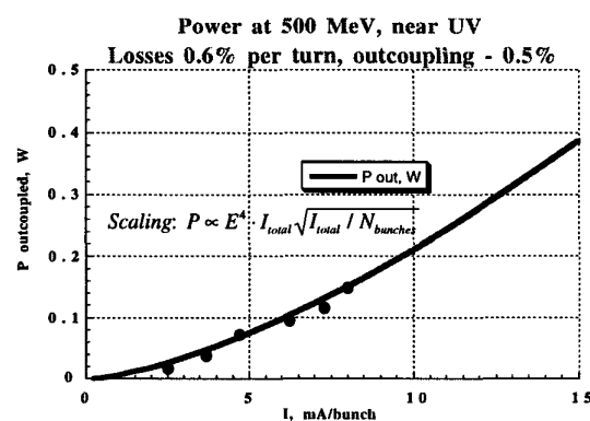
Fig. 3 Measured and predicted extracted lasing power from the OK-4 FEL. More than 80% of the power was extracted.
