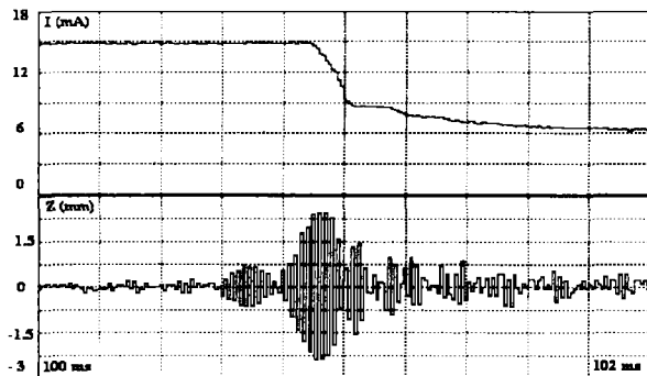
Fig. 1. The bunch head-tail instability after injection.
