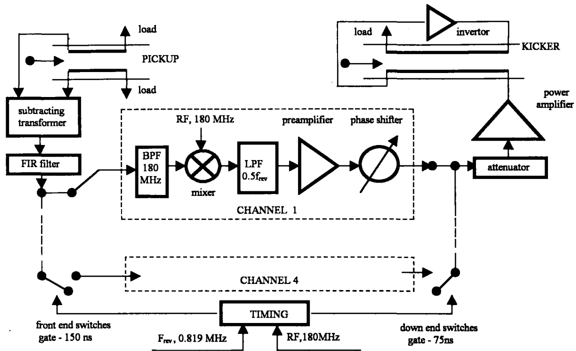
Fig.2. The feedback system blok diagram.
