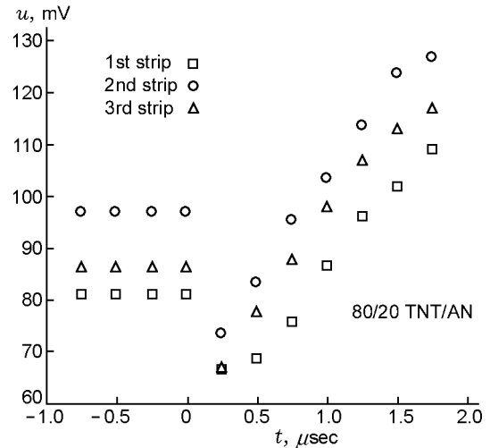
Fig. 9. Amplitudes of signals of the microstrip detector versus time (the distance between the strips is 0.4 \text{ mm} ).
