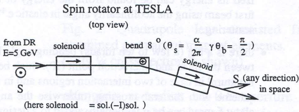
Figure 2: Scheme of the spin rotator.
