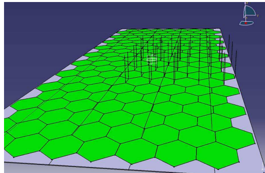
FIGURE 5.20. The mechanical structure for the ECAL proposed by the Silicon Detector group. Tungsten planes (grey) of 200 kg weight are joined to a module by rods (black). Hexagonal sensor planes (green) are placed in between the tungsten plates.
