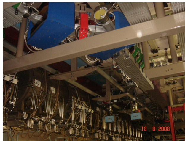
Figure 8: Bending magnets at the entrance of bypass (top). Accelerating RF cavities, vacuum chambers of two first tracks, and undulator (blue) are seen at the lower part of the picture.
