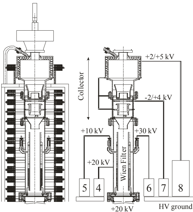
Figure 2: Collector and Wien filter.
