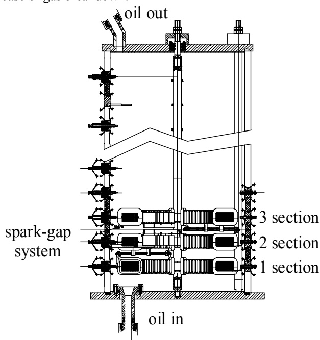
Figure 3: Transformer column.
