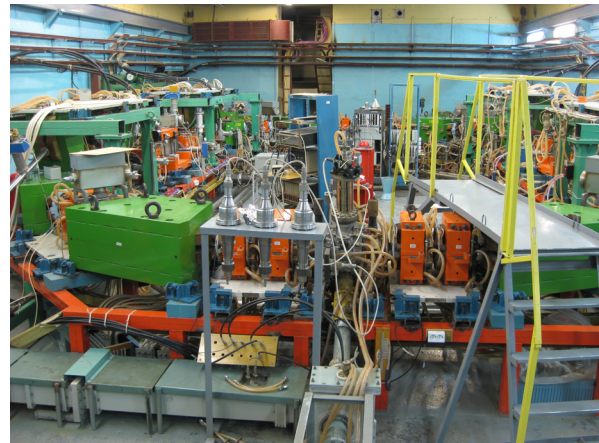
Figure 2: Damping ring.
