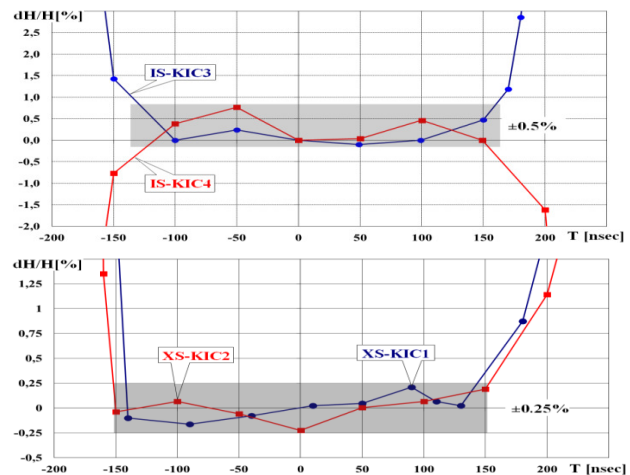
Figure 5: Shape of pulse top of injection (top) and extraction kickers (bottom).
