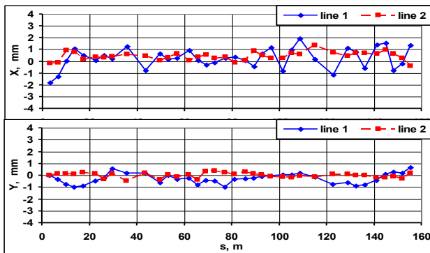
Figure 2: Horizontal and vertical orbit of beam at 200 MeV before (blue) and after (red) using the improved model.
