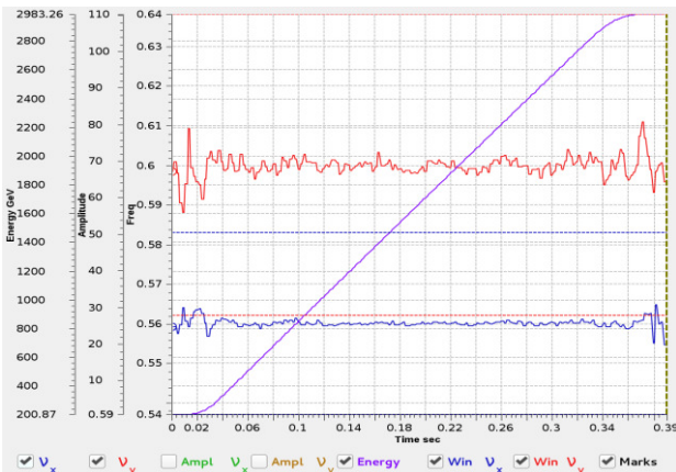
Figure 3: Horizontal (blue) and vertical (red) tunes throughout the ramp (purple).
