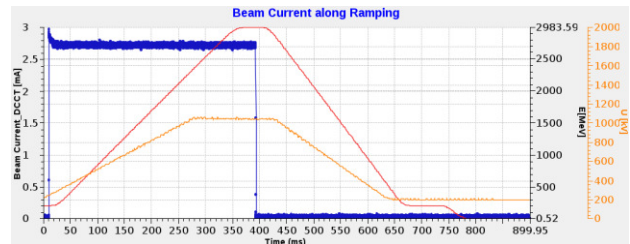
Figure 4: Booster beam current (blue); beam energy derived from dipole magnet currents (red); RF cavity voltage (orange) during 1Hz cycle.
