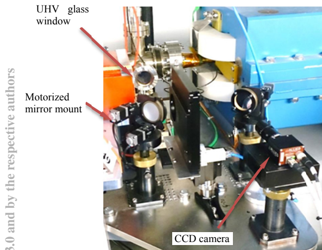
Figure 6: Image formatting optics and CCD camera installed at the booster ring.
