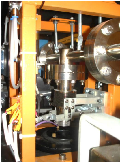
Figure 3: Beam flag at the booster ring.
