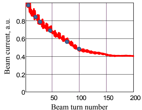
Figure 6: Beam loss because of crossing of DA.
