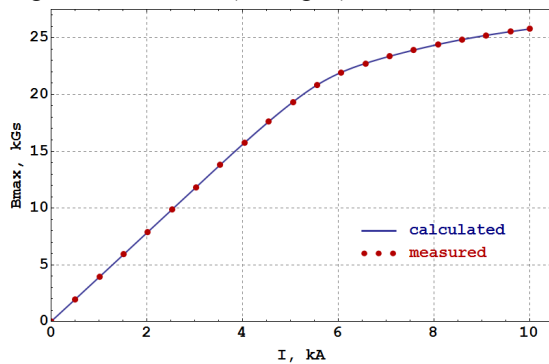
Figure 4: Dipole maximum field current dependence.
