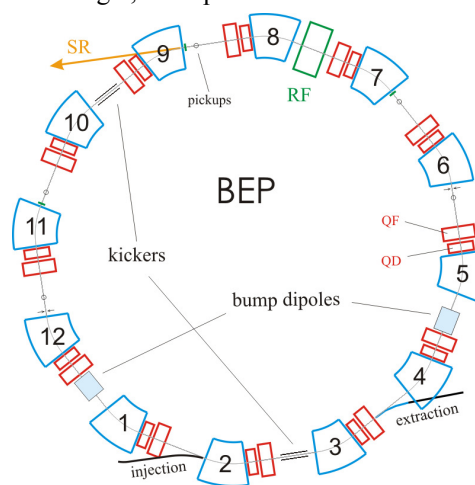
Figure 2: Booster synchrotron BEP layout.
