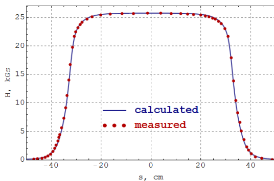
Figure 5: Field longitudinal distribution B_z(s) at 9.9 kA.
