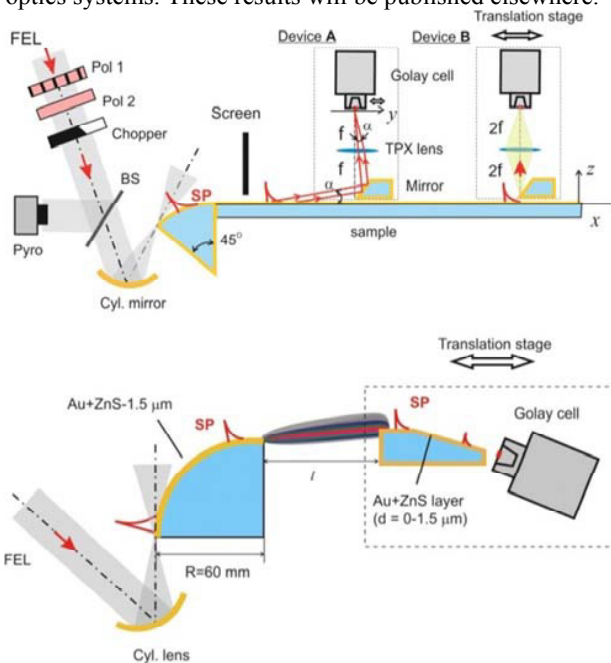
Fig. 4 Quasi-continuous optical discharge ignited by NovoFEL radiation in the focus of high-NA parabolic mirror; \lambda=130 \mu\text{m} .
