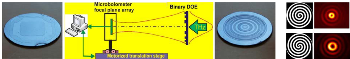
Fig. 2 Diffractive optical elements transforming Gaussian beam with wavelength \lambda_0=141 \mu\text{m} into uniformly illuminated square (left) and pencil-like beam (right). Beam shape were studied using uncooled microbolometer matrix [Dem'yanenko et al. (2008) and Dem'yanenko et al. (2011)] moved by motorized translation stage.
