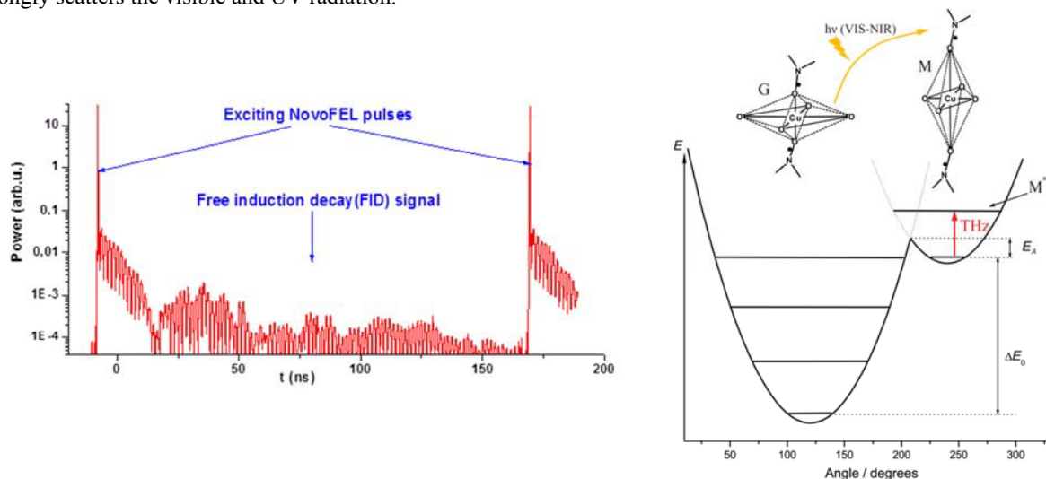
Fig. 6. Free induction decay emission of molecules of isotopic gas mixtures H^{79}Br + H^{81}Br (pressure of 0.04 Torr, pipe 1 meter long) between two exciting NovoFEL pulses, following with frequency of 5.6 MHz.
