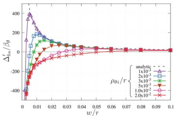
Figure 1. Plot of \Delta'_{bs} normalised to \beta_\theta as a function of w/r , for various values of \rho_{\theta i}/r . Analytic limit corresponds to \rho_{\theta i} \ll w [2].
