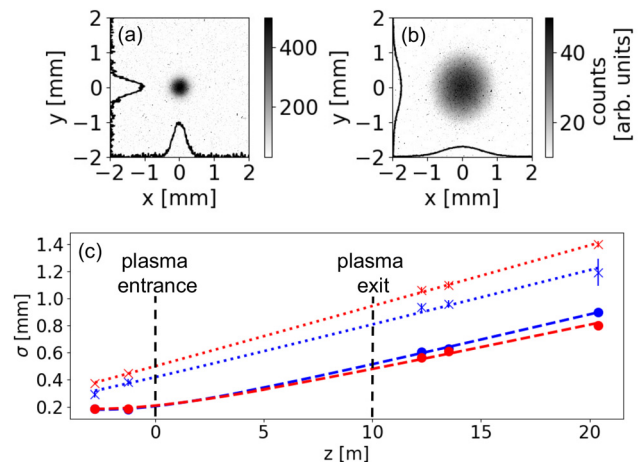
FIG. 2. Transverse, time-integrated images ( x, y ) of (a) the narrow and (b) wide bunch, at z = -1.5 m. Black lines show the projections of the transverse planes. (c) The transverse size of the bunch along the beamline \sigma_{x,y} , obtained from Gaussian fits to the transverse projections of images at the various screens with no plasma. Circles: narrow-bunch optics, crosses: wide-bunch optics, blue symbols: x -plane, red symbols: y -plane. Dashed and dotted lines: the result of the fits with the envelope equation. Plasma entrance at z = 0 , exit at z = 10 m.
