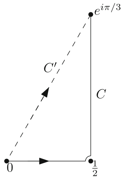
Fig. 3 Integration paths C and C' on the complex plane of y_2
