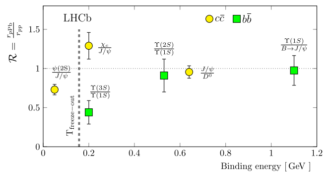
FIG. 3. Double ratio of the quarkonium state yield relative to its ground state or open heavy quark meson in pPb to pp collisions vs the binding energy of the given quarkonium state. The estimated freeze-out temperature in pPb collisions [4–6] is indicated. The details of the measurement for each data point in the figure are given in Table III.
