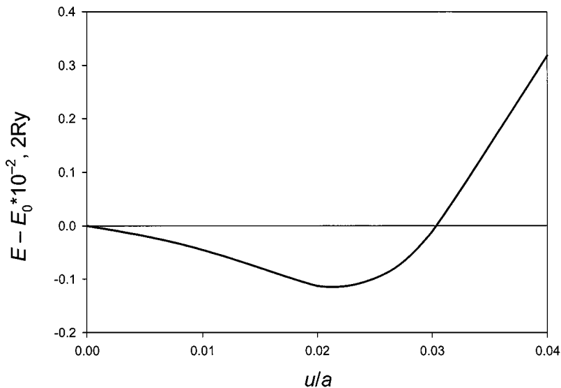
Figure 10. Energy of the crystal (per double cubic cell) as a function of fluorine atoms' displacement from their equilibrium positions in the cubic lattice. E_0 = -2148.9854 , 2Ry is the energy of undistorted phase.
