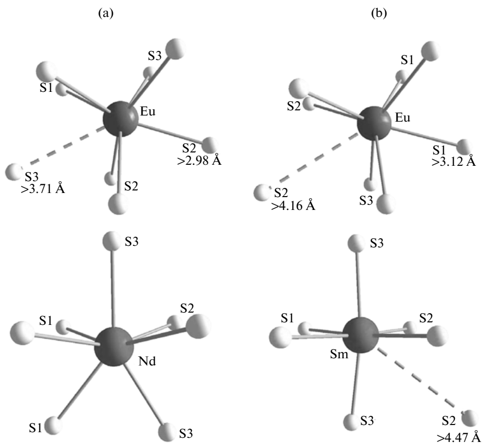
Fig. 3. Coordination of Eu and Ln in (a) \text{EuNdCu}_3 and (b) \text{EuSmCu}_3 .
