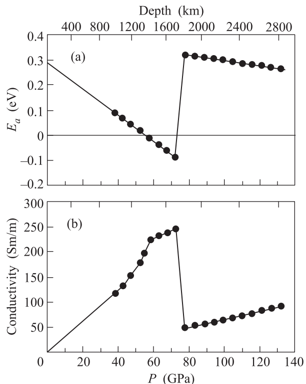
Fig. 2. Pressure dependence of the activation energy (a) and the depth profile of conductivity (b). The decrease at small pressure with closure of the gap at 56 GPa is due to the Mott–Hubbard transition. The reentrant metal-insulator transition at 77 GPa results from the spin crossover. Negative E_a interval of pressure corresponds to the metal region in the Fig. 1 along the bold dash line
