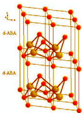
Fig. 2. Schematic representation of Fe–O–Fe bonds in the defective phase ABABA by notation in Jansen et al. [14]; small circles represent O and OH ligands, and large circles represent Fe^{3+} ions
