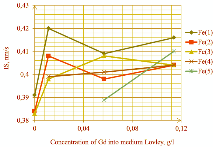
Fig. 5. IS - isomer chemical shift of nonequivalent iron positions relative to \alpha -Fe in the bacterial ferrihydrite as a function of gadolinium concentration in the Lovley medium
