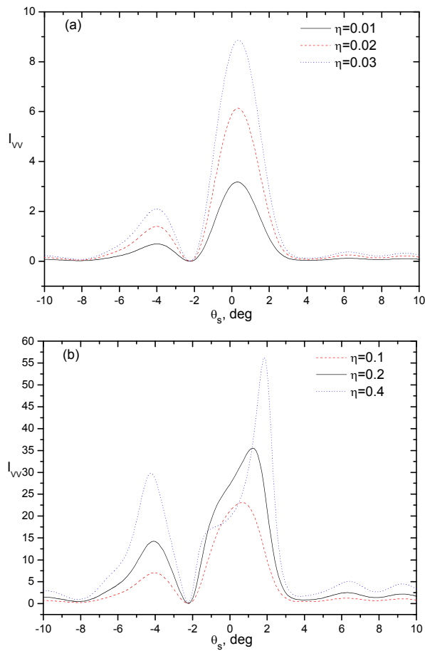
Fig. 4. Dependence of I_{vv} -component of the light intensity scattered by a monolayer of spherical LC droplets with inhomogeneous boundary conditions at different values of the filling factor \eta = 0.01, 0.02, 0.03 (a), \eta = 0.1, 0.2, 0.4 (b). No field applied. W = 50\% , \lambda = 0.633 \mu\text{m} , n_o = 1.531 , n_e = 1.717 , n_p = 1.532 , \eta = 0.5 , a = 5 \mu\text{m} , \alpha = 0 , \varphi_s = 0 .
