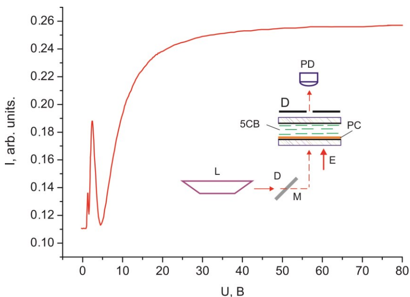
Figure 3. Voltage dependence of intensity I of monochromatic light passed through the 30 \mu\text{m} thick planar 5CB layer with domains formed on the PC surface.
