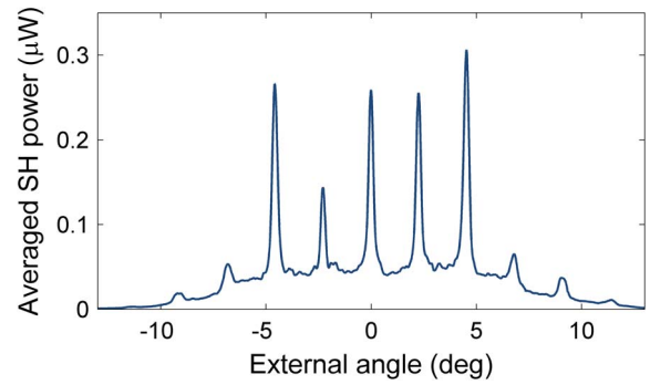
Fig. 2. Measured angular distribution of averaged SH power for FF incidence angle \sim 3 mrad.
