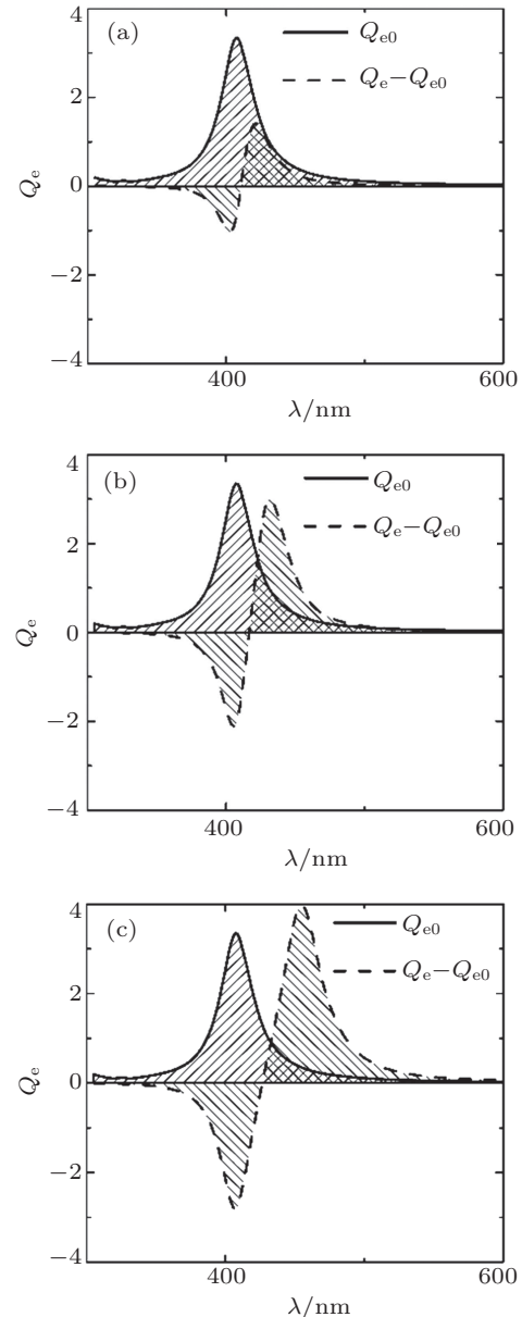
Fig. 4. Initial and differential extinction spectra of dimer ( R_1 = R_2 = 5 \text{ nm} ) corresponding to different magnitudes of photomodification factor ( \mu ): (a) -0.4 , (b) -1 , (c) -1.6 . Shading shows the numerator and denominator of Eq. (1).
