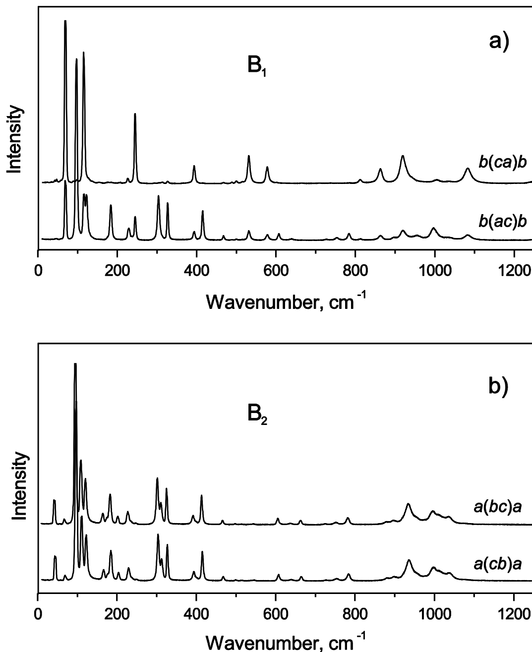
Figure 3. Raman spectra of the \delta -BiB 3 O 6 crystal at: a) a(bc)a b) a(cb)a
