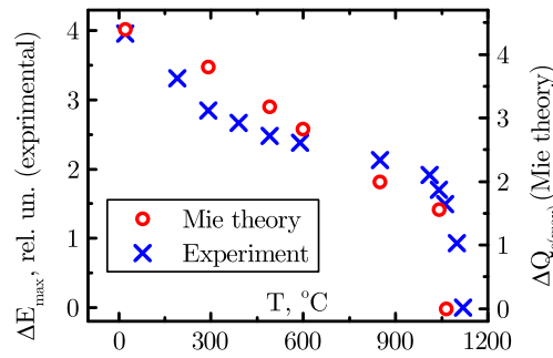
Fig. 3. Temperature dependence of SPR amplitude of Au nanoparticles in experiment \Delta E_{max} and in calculations \Delta Q_{e(max)} .
