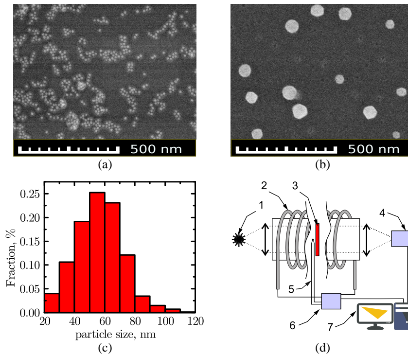
Fig. 1. SEM image of gold nanoparticles on the quartz substrate before (a) and after (b) first heating and cooling cycle in the furnace; (c) particle diameter distribution function after first heating and cooling cycle (averaged over several images); (d) experimental setup 1 — light source (250 W halogen lamp), 2 — heating element, 3 — sample, 4 — high-speed-spectrometer, 5 — K-type thermocouple, 6 — temperature controller, 7 — PC.
