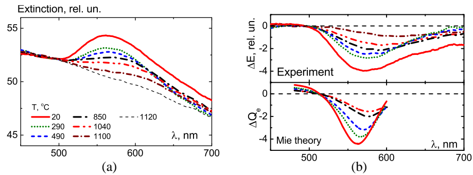
Fig. 2. (a) — experimental evolution of Au nanoparticle extinction spectrum and reduction of the amplitude of SPR from room to melting temperatures 20–1120 °C (see the legend); (b) — the same evolution of differential spectra and comparison with calculations based on the Mie theory using dielectric constants for gold at same temperature values. \Delta E = E(1120\text{ °C}) - E(T) and \Delta Q_e = Q_e(1064\text{ °C}) - Q_e(T) .
