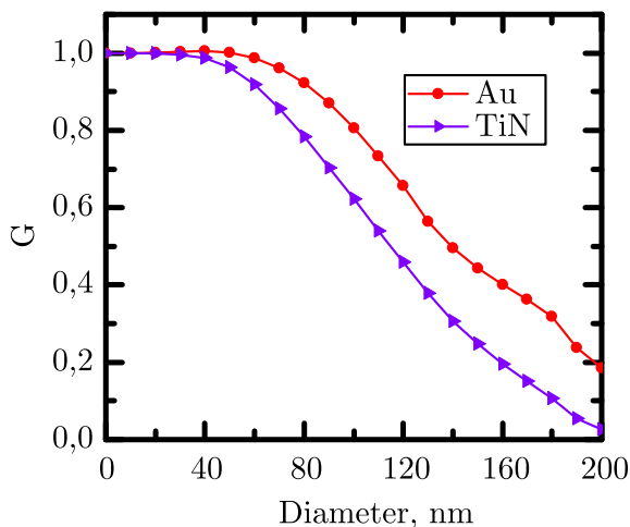
Fig. 4. The enhancement Factor G with different TiN and Au nanoparticle diameters.
