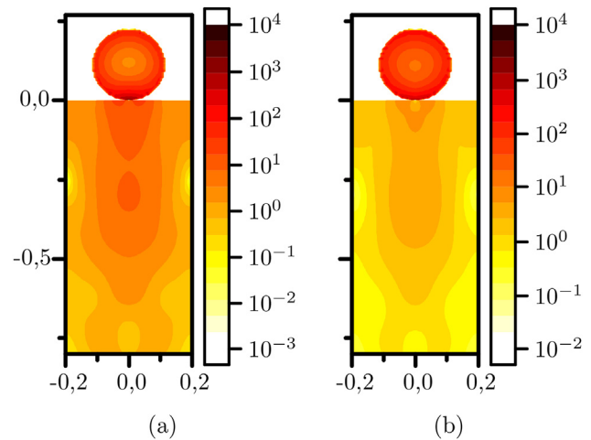
Fig. 5. The relative absorption distribution per unit volume in silicon with Au — (a) and TiN — (b).
