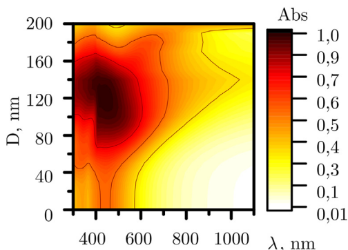
Fig. 2. The absorption Spectra for different particle Diameter — Abs( \lambda, D ).
