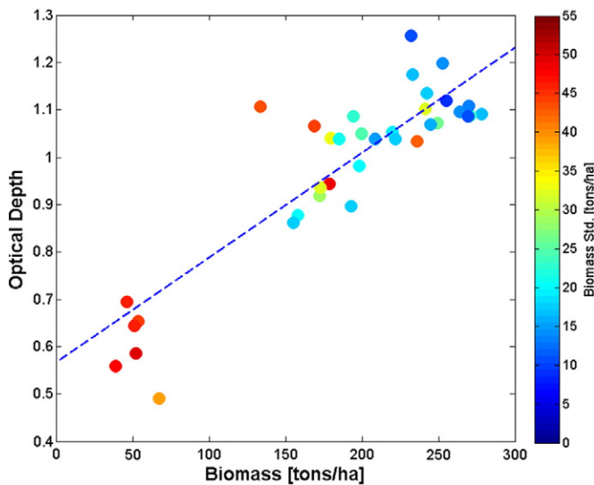
Fig. 10. Scatterplot of SMOS retrieved \tau vs. forest biomass measured in forest pixels of Peru and Columbia. Color codes indicate the standard deviation of measured biomass within SMOS pixels ( R^2 = 0.74 ) (Vittucci et al., 2016).
