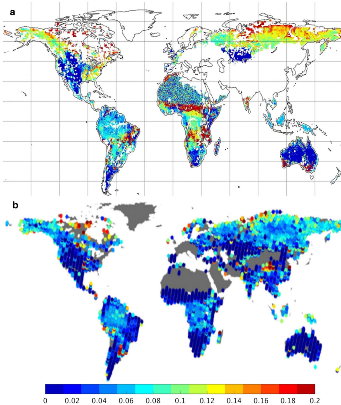
Fig. 7. Global map of effective scattering albedo at L-band retrieved from the (a) SMOS TB data (SMAP L4_SM product; De Lannoy et al., 2014) and (b) Aquarius (Konings et al., 2016) observations.
