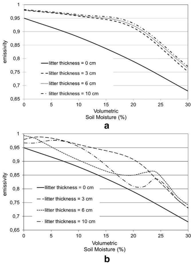
Fig. 11. Emissivity of a soil-litter system as a function of soil moisture for several values of the litter thickness (0, 3, 6 and 10 cm). Computations were made using an incoherent (a) and a coherent (b) model (Demontoux et al., 2008).
