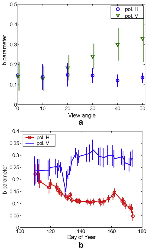
Fig. 5. Dependence of the b parameter on (a) incidence angle and polarization and (b) Day of Year (well-developed wheat canopy, PORTOS-93 experiment; adapted from Wigneron et al., 2004).
