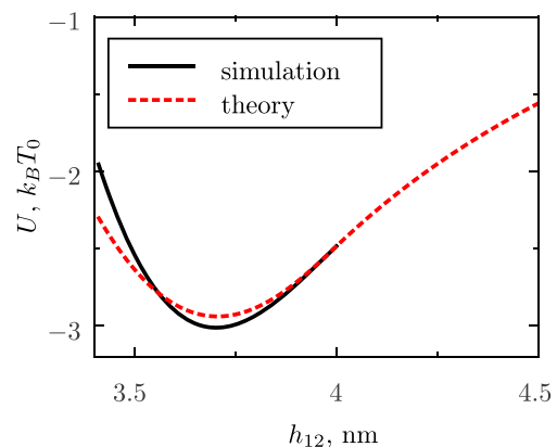
Fig. 5 Dependence of the total van der Waals and elastic interaction energy on interparticle gap. The energy of elastic interaction was calculated using Eq. 4 (dashed line) and by the finite elements method FEM (solid line). The van der Waals interaction energy in both cases was calculated with Eq. 4 using following parameters: E_{el} = 10^7 N/m^2 (dashed line), E_{el} = 2.07 \cdot 10^7 N/m^2 (solid line), r_0 = 10 nm, and h_0 = 2 nm
