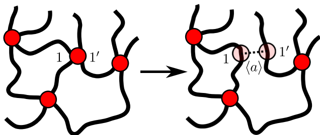
Fig. 6 Local section of a polymer network with a broken bond 1 – 1'(node)
