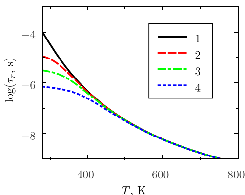
Fig. 8 Dependence of the relaxation time on temperature for different values of E_{el}(T_r) : 1 — 5.8 \cdot 10^3 N/m 2 , 2 — 10^6 N/m 2 , 3 — 10^7 N/m 2 , 4 — 10^8 N/m 2
