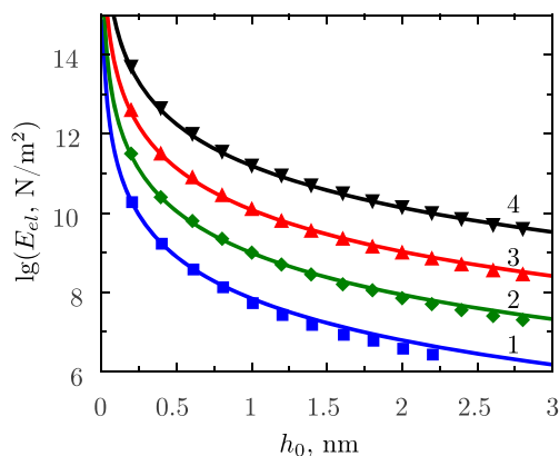
Fig. 3 Dependence of the effective elasticity modulus of a polymer adlayer on its thickness (points are numerical values, solid lines are approximations for particles with different radii: 1 — r_0 = 5\text{ nm} , 2 — r_0 = 10\text{ nm} , 3 — r_0 = 15\text{ nm} , 4 — r_0 = 25\text{ nm} ). For ease of perception, curves 2, 3, and 4 are successively shifted upwards by one vertical scale step
