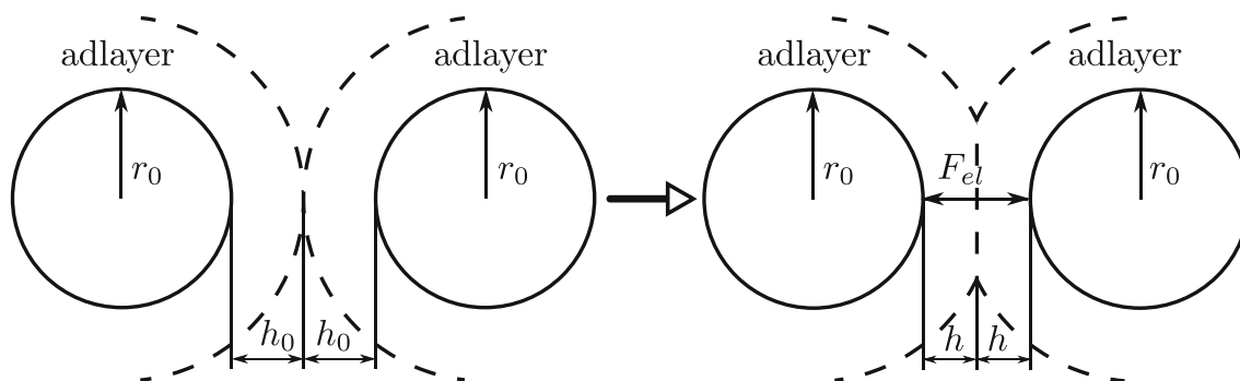
Fig. 1 Contact deformation of adlayers of two identical particles
