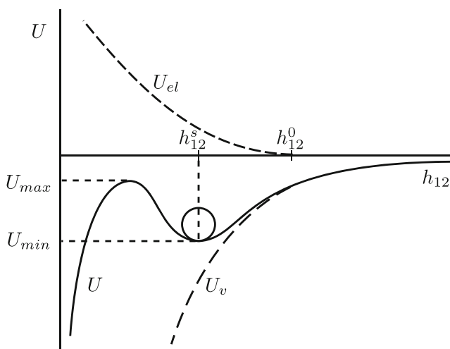
Fig. 2 The scheme of capture of a particle into a potential well
