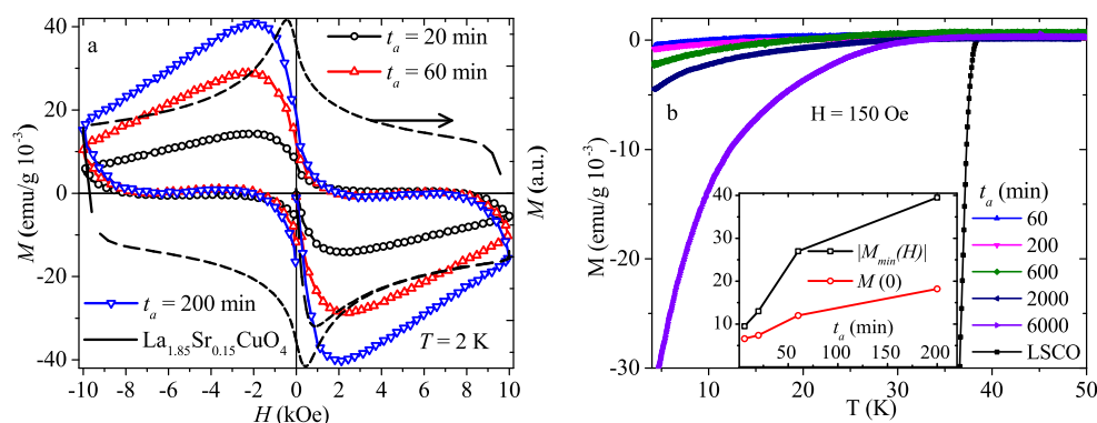
Fig. 4 Dependencies of the magnetization M on the magnetic field H (a) and temperature dependencies of the magnetization M(T) in the ZFC regime (b). Inset shows the trapped field M(0) and the absolute value of the magnetization minimum |M_{\min}|
