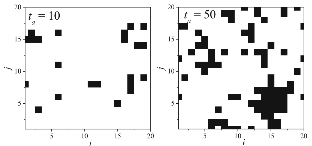
Fig. 6 Simulation results. Black sections denote pinning centers (the normal clusters, surrounded by the closed superconducting contour)
