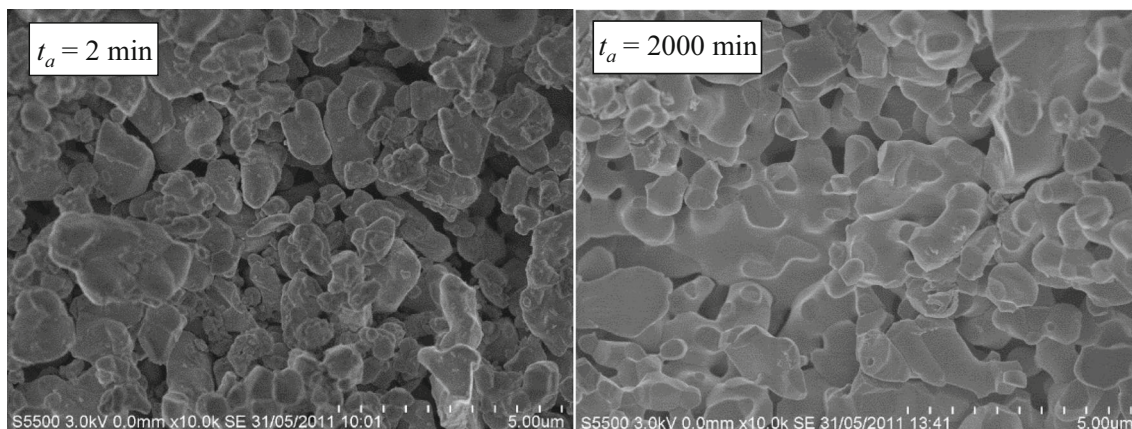
Fig. 1 Microphotographs of the samples with the annealing time t_a = 2 and 2000 min
