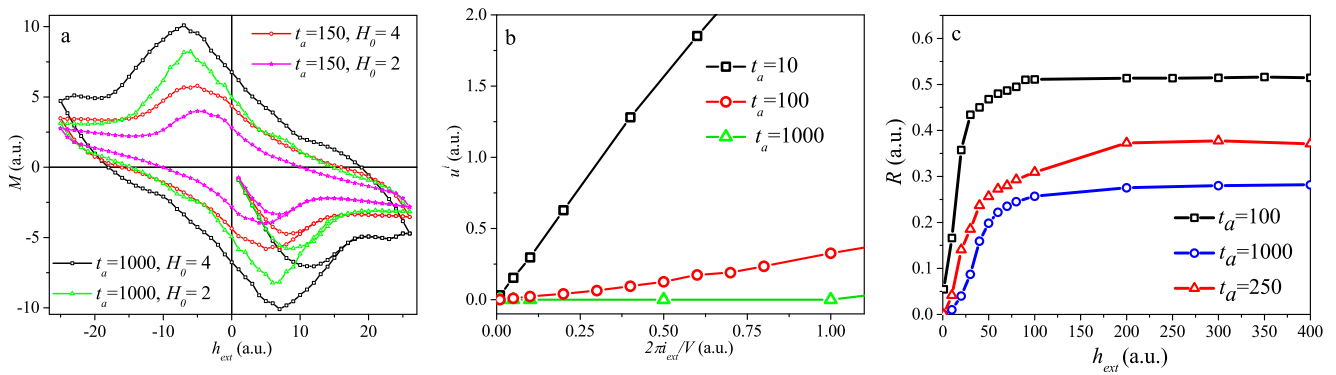
Fig. 7 Computed curves for some t_a : magnetization loops with different H_0 (a), I - V curves (b), the resistance R versus the external magnetic field H (c)
