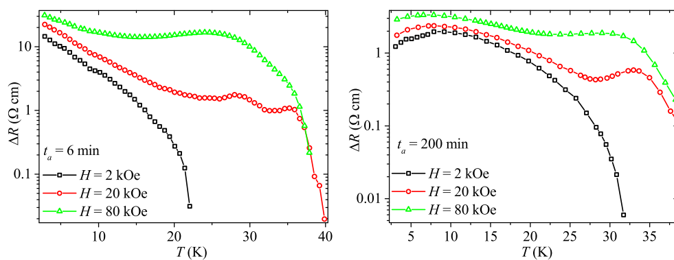
Fig. 3 Temperature dependencies of the additional resistance \Delta R(T) = R(T, H) - R(T, H = 0) for t_a = 6 and 200 min
