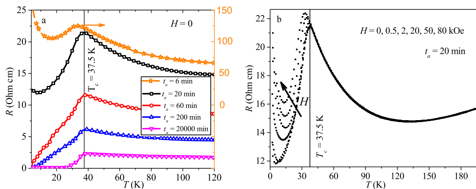
Fig. 2 Temperature dependencies of the resistance of samples with different annealing time t_a (a) and the dependencies for t_a = 20 min in magnetic fields (b)
