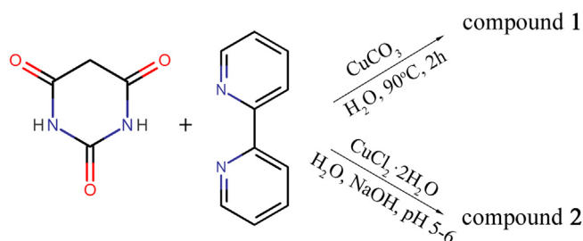
Scheme 1. Synthesis routes of 1–2.
