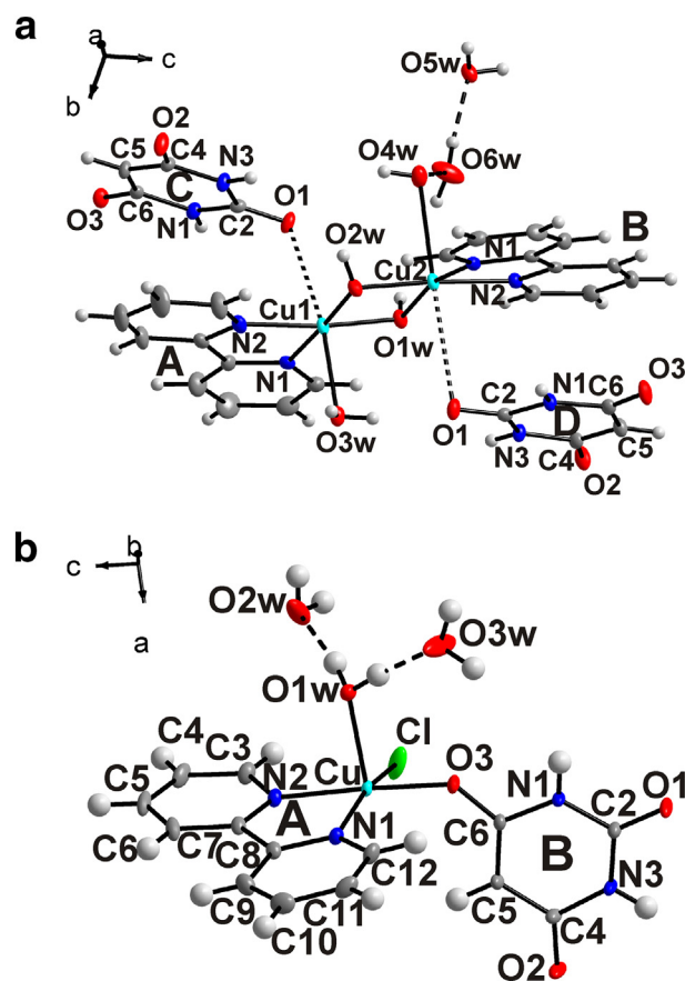
Fig. 1. The asymmetric unit of the 1 (a), 2 (b) unit cell. Symmetry independent, different molecules are marked by A, B, C, D labels. Some most important atoms in the asymmetric unit are labeled. The intermolecular hydrogen bonds are represented by dashed lines. The ellipsoids are drawn at the 50% probability level, except for the hydrogen atoms represented by spheres.
