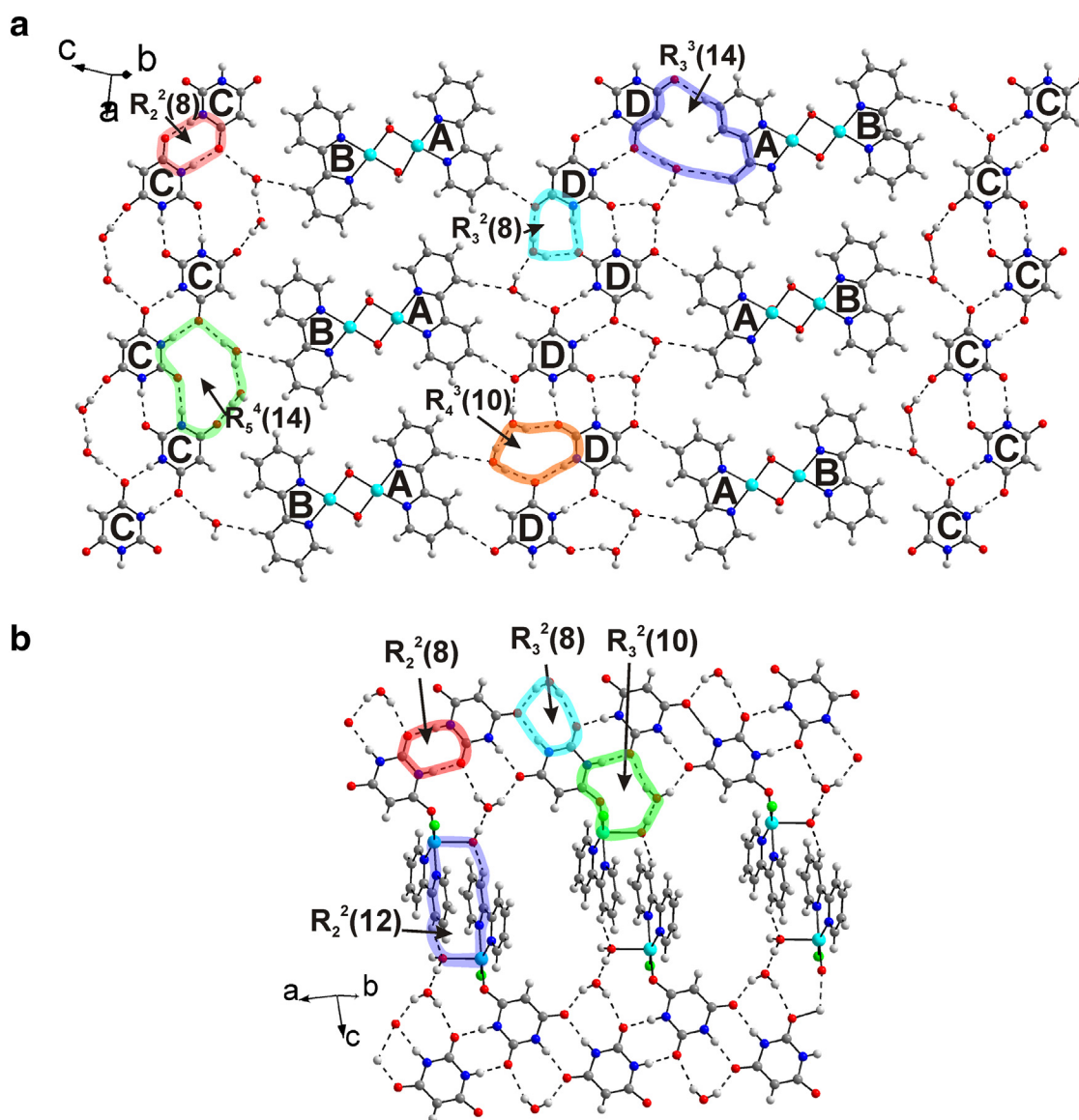
Fig. 2. Hydrogen bonding in 1 (a) and 2 (b). The H-bonds are marked by dashed lines, the H-bond motifs are marked by circles. Different ions/molecules are marked by A, B, C, D labels.
