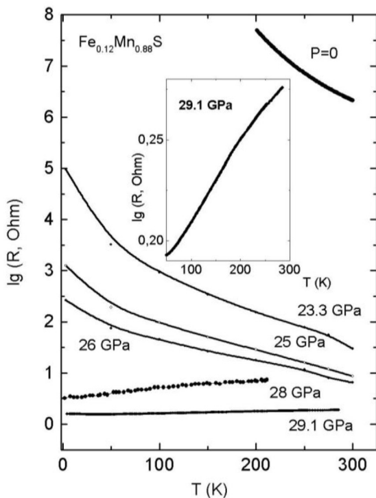
Fig. 4. The temperature dependences of the resistance at the hydrostatic pressure for \text{Fe}_x\text{Mn}_{1-x}\text{S} with X = 0.12 . Insert: P = 29.1 GPa.
