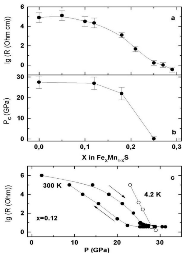
Fig. 5. The chemical (a, under ambient conditions) and hydrostatic pressure (c, for X = 0.12 ) dependences of the room temperature resistivity for \text{Fe}_x\text{Mn}_{1-x}\text{S} . (b) The critical pressure P_c vs X at room temperature. (a): The error of the data is caused by the fluctuation of the chemical composition of the samples with the same X (the actual chemical composition of these samples fluctuated within X \pm 0.02 ).
