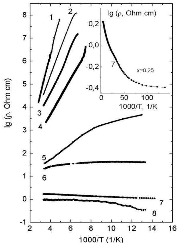
Fig. 2. The temperature dependences of the resistivity for \text{Fe}_x\text{Mn}_{1-x}\text{S} with X (a) X = 0 (1), 0.1 (2), 0.15 (3); 0.18 (4); 0.21 (5); 0.23 (6), 0.25 (7), 0.27 (8) under ambient conditions. Insert: the temperature dependences of the resistivity for the \text{Fe}_x\text{Mn}_{1-x}\text{S} with X = 0.25 . The kink in the curve 4 is connected with the change of the measuring current due to the nonlinearity of the current-voltage characteristics below 130 K.
