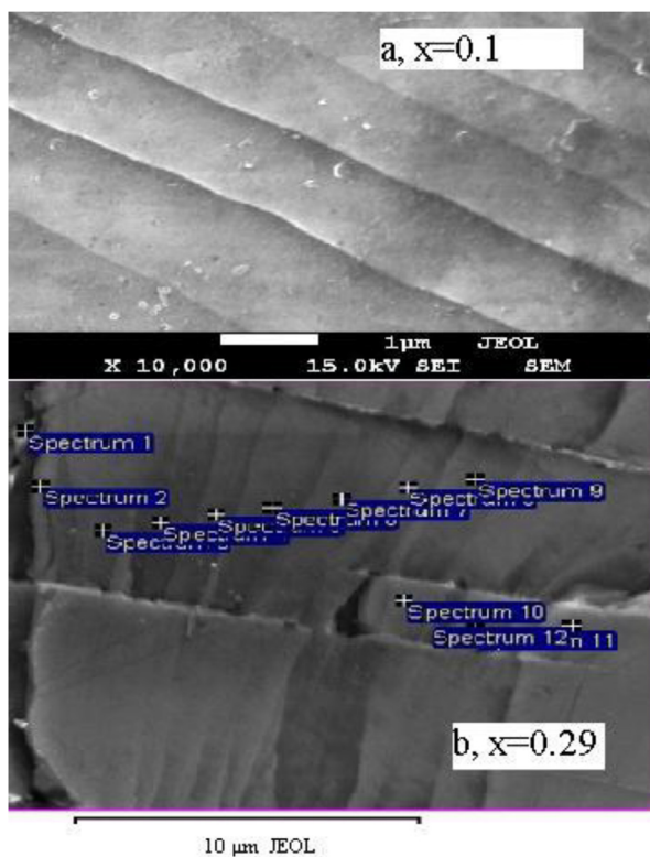
Fig. 1. The SEM images of the single crystal \text{Fe}_x\text{Mn}_{1-x}\text{S} with x = 0.1 (a) and x = 0.29 (b).
