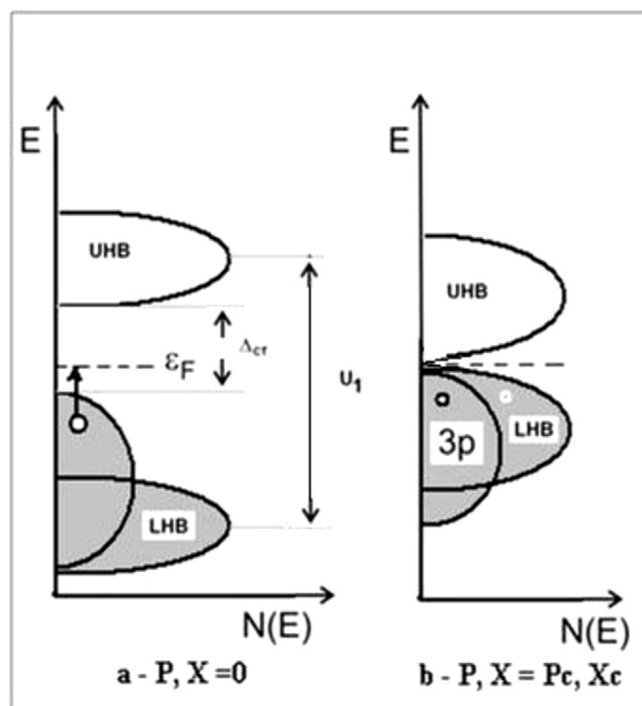
Fig. 6. The schematic band structure of the MnS under the chemical and hydrostatic pressures.
