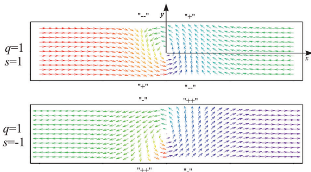
Figure 2. Example of the magnetization distribution in the vortex wall at different combinations of parameters q and s at \delta_w = L and \delta_c = 0.2\delta_w .
