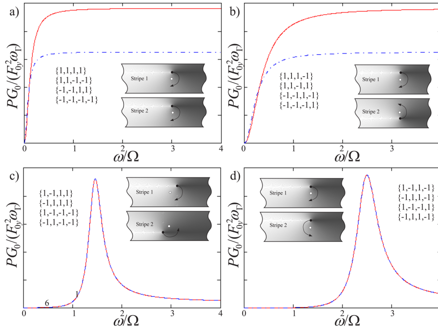
Figure 6. Dependence of the absorbed power (arb. units) on the frequency of ac field applied along the x axis. The curves are built for the same parameters as in Figure 5.
