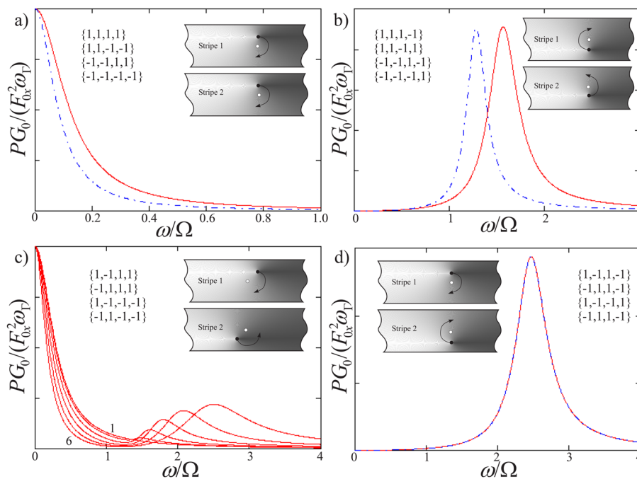
Figure 5. Dependence of the absorbed power (arb. units) on the ac field frequency. The ac field is applied along the y axis. The curves are plotted for the parameters \omega_y = \Omega , \omega_x = \omega , \omega_r = 0.1 , and h = 0.1 . a, b) Power for the case of a dc field applied antiparallel to the z axis (dashed lines). c, d) Dc field applied parallel and antiparallel to the z axis. c) Set of curves 1–6 at dc fields of h = 0 \dots 0.5 with a step of \Delta h = 0.1 . Inset: polarity and chirality combinations \{p_1, p_2, q_1, q_2\} for the vortex walls and phases and directions of the vortex cores. Closed circles show the cores and open circles, the origins of coordinates.
