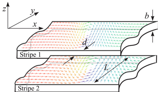
Figure 1. Model of a pair of parallel stripes.
