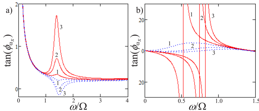
Figure 7. Dependence of the tangent of x -coordinate phase of the magnetic vortex core in stripe 1 (solid curves) and stripe 2 (dotted lines). Curves 1, 2, and 3 are built for perpendicular fields of h_1 = 0.01 , h_2 = 0.05 , and h_3 = 0.1 , respectively. a) Plot for the ac field applied along the y axis, and b) plot for the ac field applied along the x axis.
