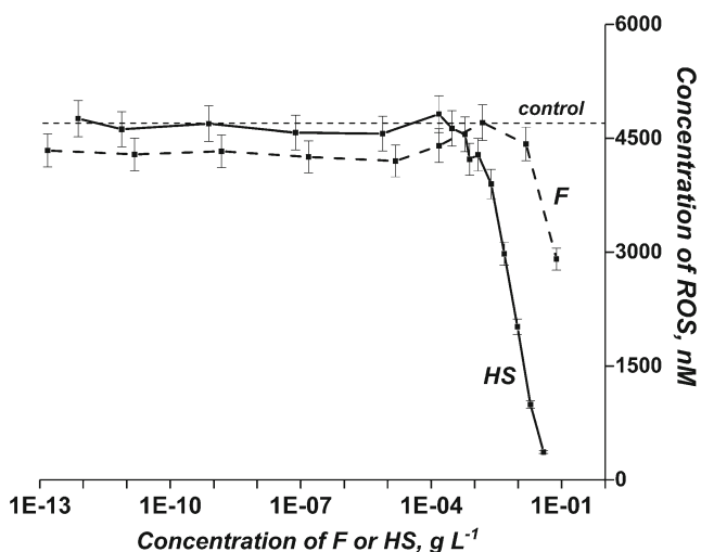
Fig. 3 Concentration of ROS vs. concentrations of bioactive compounds: humic substances (HS) and fulleranol (F). Chemiluminescence assay
