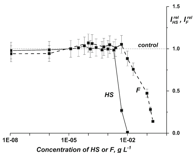
Fig. 2 Relative bioluminescence intensity I^{rel} at different concentrations of bioactive compounds: humic substances (HS) and fullerol (F). Enzymatic assay
