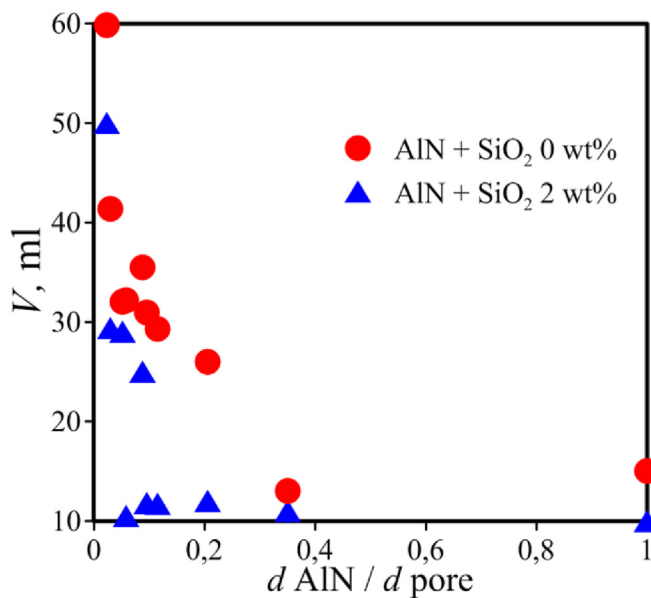
Fig. 11. The filtration loss of drilling fluid containing SiO 2 nanoparticles 5 nm in size at a concentration of 2 wt% depending on the ratio of the AlN microparticle size at the concentration of 2 wt% to the average pore size of the filter, defined by the mercury.
