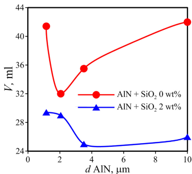
Fig. 10. The filtration loss of drilling fluid depending on the size of microparticles of AlN with 2 wt% containing 2 wt% of SiO 2 nanoparticles 5 nm in size for the ceramic filter with an average pore size of 20 μm (by air).
