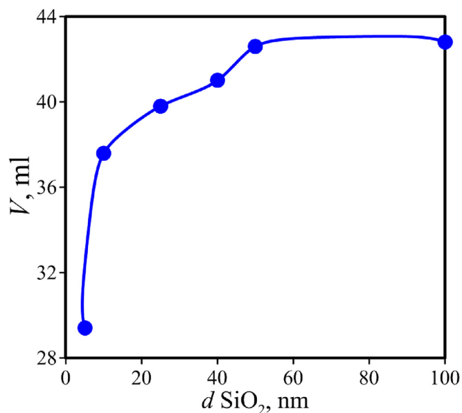
Fig. 9. Filtration loss of microsuspension containing AlN microparticles 1\ \mu\text{m} in size at a concentration of 2 wt% depending on the average size of SiO 2 nanoparticles at a concentration of 2 wt% for a ceramic disk with a pore diameter of 20\ \mu\text{m} (by air).
