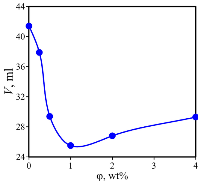
Fig. 3. Filtration loss depending on the SiO 2 nanoparticle concentration.
