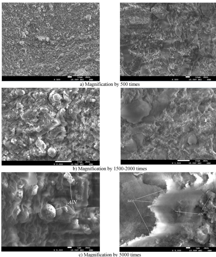
Fig. 4. The SEM images of the filter cake of the drilling fluid containing 2% of AlN microparticles 1 μm in size without the addition of nanoparticles (left images), and with the addition of SiO 2 nanoparticles (right images).
