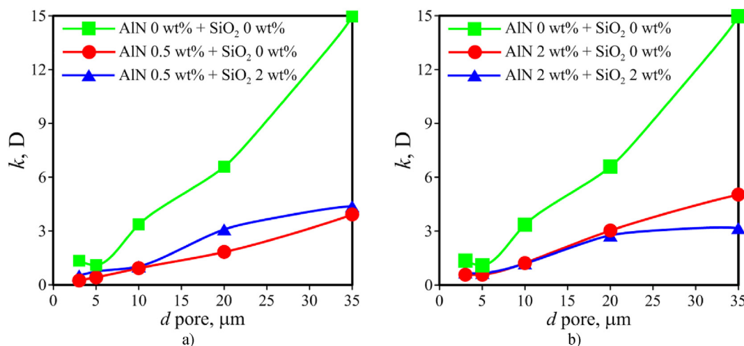
Fig. 8. The permeability of ceramic filters depending on the size of their pores (by air) after filtration through them of microsuspension containing AlN microparticles 1\ \mu\text{m} in size and SiO 2 nanoparticles 5\ \text{nm} in size.
