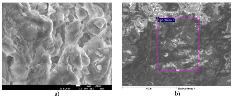
Fig. 1. SEM micrograph of clay particles: in secondary electrons (a), with spectrum marker (b).
