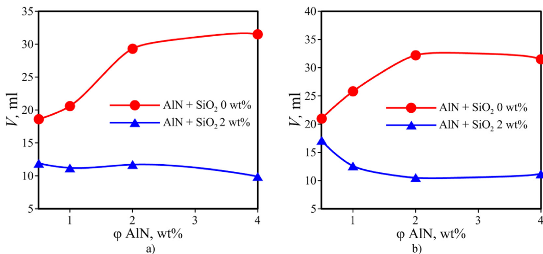
Fig. 6. Filtration loss depending on the concentration of AlN microparticles with a size of 1 \mu\text{m} without and with the addition of 2 wt% of nanoparticles 5 nm in size for the ceramic filters with pore sizes equal to 3 \mu\text{m} (a) and 10 \mu\text{m} (b) (by air).
