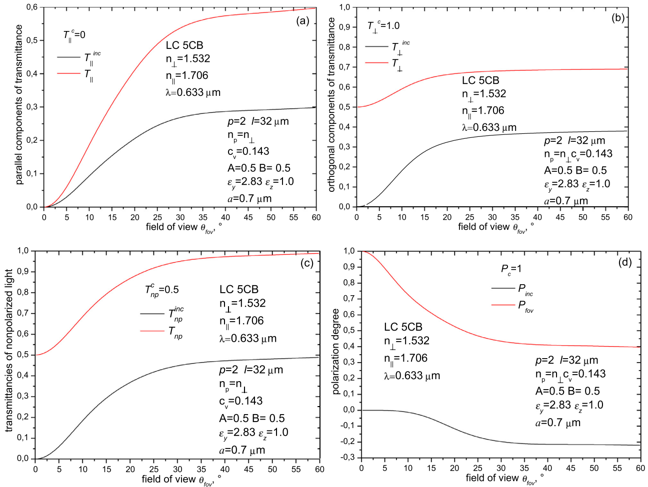
Fig. 17. The dependences of the transmittance for parallel (a) and orthogonal (b) components of scattered light, the transmittance for unpolarized incident light (c), and the polarizing degree (d) on the field of view angle \theta_{fov} . The structure within LC droplets is monodomain. The stretching ratio of the film is p=2 . n_p = n_{\perp} = 1.532 . The wavelength of incident light \lambda = 0.633 \mu\text{m} . a = 0.7 \mu\text{m} .
