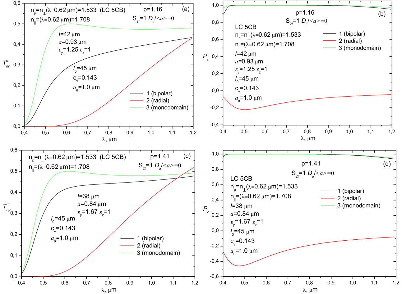
Fig. 3. The spectral dependences of the coherent transmittance T_{np}^c(\lambda) (a, c) and polarization degree P_c(\lambda) of the forward-transmitted light (b, d) at the different stretching factor p of the PDLC films containing droplets with the bipolar (curves 1), radial (curves 2) and monodomain (curves 3) y-configuration of LC director. n_p = n_{\perp} = 1.533 at \lambda = 0.62 \mu\text{m} .
