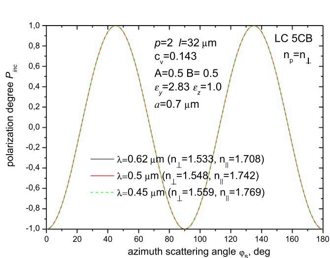
Fig. 12. Dependences of the polarization degree P_{inc} of scattered light on the azimuthal scattering angle \varphi_s in the condition of the equality of the refractive index n_p of polymer matrix and ordinary refractive index n_{\perp} of 5CB at \lambda = 0.62, 0.5, 0.45 \mu\text{m} . The stretching ratio of film is p=2 . The structure within LC droplets is monodomain. a=0.7 \mu\text{m} .
