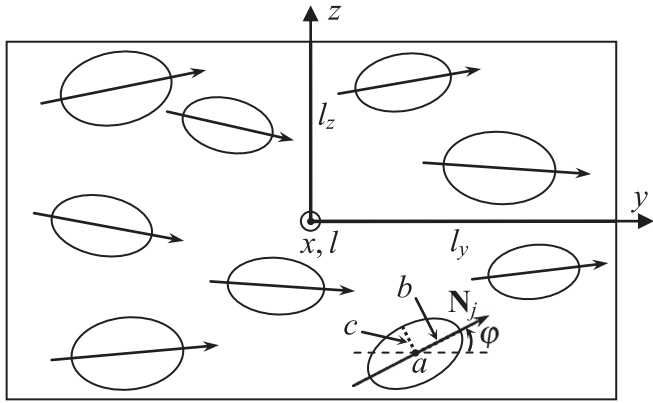
Fig. 2. Scheme of the PDLC layer structure under stretching along y axis of the laboratory coordinate system (x, y, z) . The (y, z) plane coincides with the layer-front surface. The x axis is directed along the normal to PDLC layer; \varphi is the orientation angle of optical axis \mathbf{N}_j of an individual droplet; l and l_y, l_z are the thicknesses of stretched layer and its linear sizes along y, z axes; a, b, c are the semi-axes of elongated ellipsoidal droplets. The a semi-axes are oriented along x axis and b, c semi-axes are aligned in the (y, z) layer plane. The layer is normally illuminated by unpolarized light along x axis.
