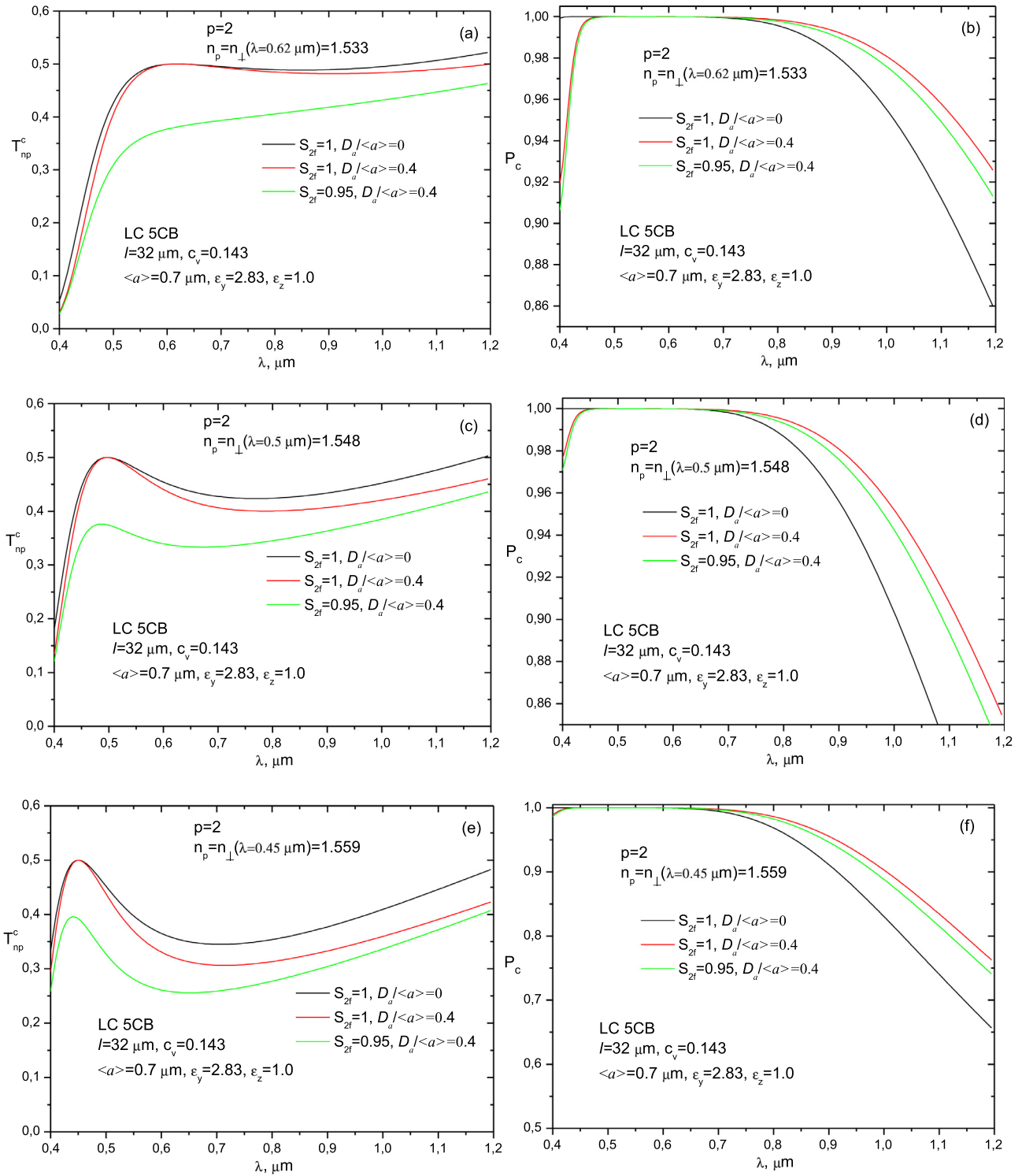
Fig. 8. The spectral dependences of coherent transmittance T_{np}^c of PDLC film (a, c, e) illuminated by unpolarized incident light and the polarization degree P_c (b, d, f) of the forward-transmitted light in condition of equality of the polymer refractive index n_p and the ordinary refractive index n_{\perp} of 5CB at \lambda = 0.62, 0.5 and 0.45 \mu\text{m} . The LC structure inside the droplets is monodomain. The stretching ratio of film is p=2 . The average size of droplet lateral semiaxis a is \langle a \rangle = 0.7 \mu\text{m} . The anisotropy parameters of droplets are \epsilon_y = 2.83 , and \epsilon_z = 1.0 . The order parameters of film are S_{2f} = 1 and 0.95 . Gamma-distribution of droplet sizes. The variation coefficients are D_a/\langle a \rangle = 0 and 0.4 .
