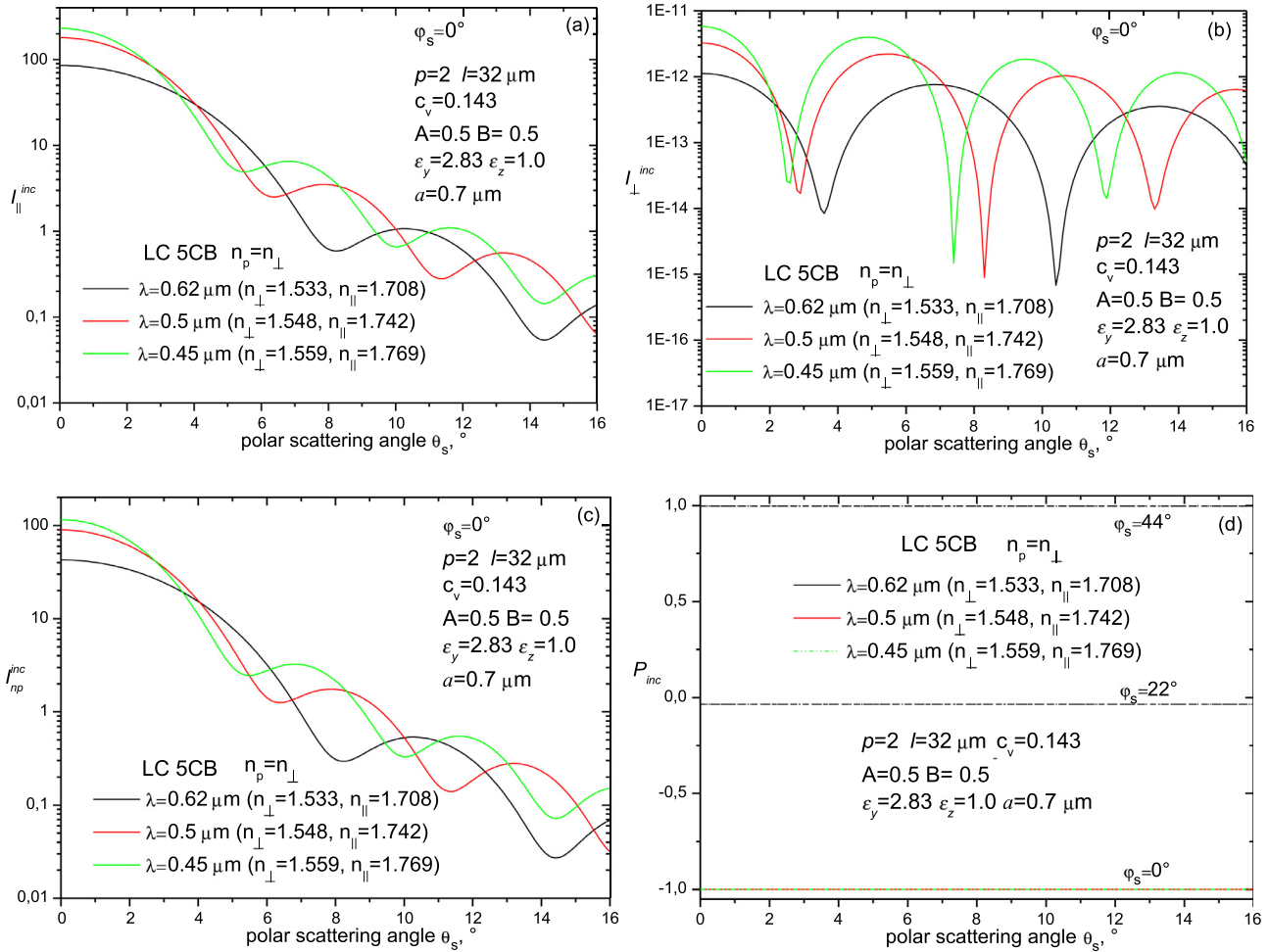
Fig. 11. Angular distribution of the parallel I_{\parallel}^{inc}(\theta_s) (a) and orthogonal I_{\perp}^{inc}(\theta_s) (b) to the stretching axis intensity components, the intensity I_{np}^{inc}(\theta_s) (c), and the polarization degree P_{inc}(\theta_s) (d) of scattered light for the refractive index n_p of polymer matrix equal to the ordinary refractive index n_{\perp} of 5CB at \lambda = 0.62, 0.5, 0.45 \mu\text{m} . The stretching ratio of film is p=2 . The structure within LC droplets is monodomain. a=0.7 \mu\text{m} .
