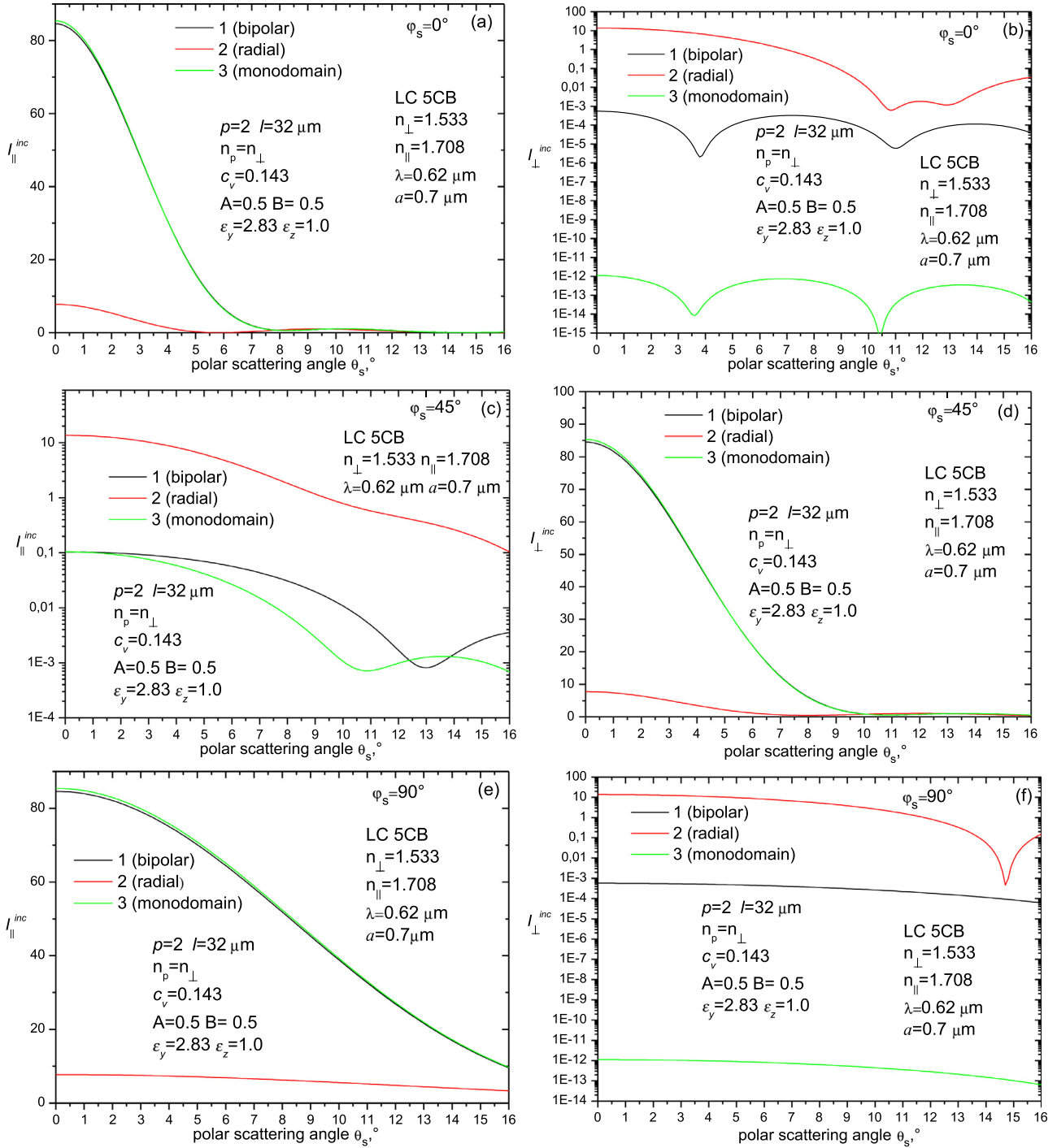
Fig. 9. The dependences of parallel (to the stretching axis) I_{||}^{inc}(\theta_s) (a, c, e) and orthogonal I_{\perp}^{inc}(\theta_s) (b, d, f) components of scattered light intensity on the polar scattering angle \theta_s at different azimuthal scattering angles \varphi_s . PDLC film was double-stretched ( p=2 ) at homogeneous (1, 2) and inhomogeneous (3) surface anchoring. n_p = n_{\perp} = 1.533 at \lambda = 0.62 \mu\text{m} .
