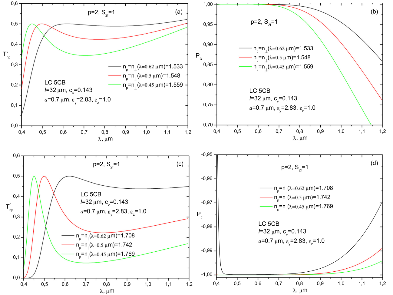
Fig. 6. The dependences of coherent transmittance T_{np}^c of PDLC film (a, c) and polarization degree P_c (b, d) of the forward-transmitted light on the wavelength \lambda of incident unpolarized light for the polymer refractive indices n_p equaled to the ordinary n_{\perp} (a, b) and extraordinary n_{\parallel} (c, d) refractive indices of 5CB at \lambda = 0.62, 0.5 and 0.45 \mu\text{m} . Monodisperse droplets with the monodomain LC structure and oriented optical axes (the film order parameter S_{2f} = 1 ). The stretching ratio of film is p=2 , the droplet lateral semiaxis is a=0.7 \mu\text{m} , the film thickness is l=32 \mu\text{m} , the volume filling factor of PDLC film is c_v = 0.143 , the anisotropy parameters of LC droplets are \epsilon_y = b/a = 2.83 , \epsilon_z = c/a = 1.0 (where b is the droplet semiaxis along the stretching direction, a is the droplet semiaxis along the normal to the film, c is the lateral semiaxis in the film plane).
