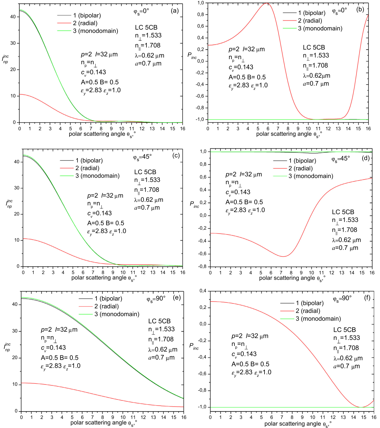
Fig. 10. The dependences of intensity I_{np}^{inc}(\theta_s) (a, c, e) and polarization degree P_{inc}(\theta_s) (b, d, f) of scattered light on the polar scattering angle \theta_s at different values of azimuthal scattering angle \varphi_s . PDLC film was double-stretched ( p=2 ) at homogeneous (1, 2) and inhomogeneous (3) surface anchoring. n_p = n_\perp = 1.533 at \lambda = 0.62 \mu\text{m} .
