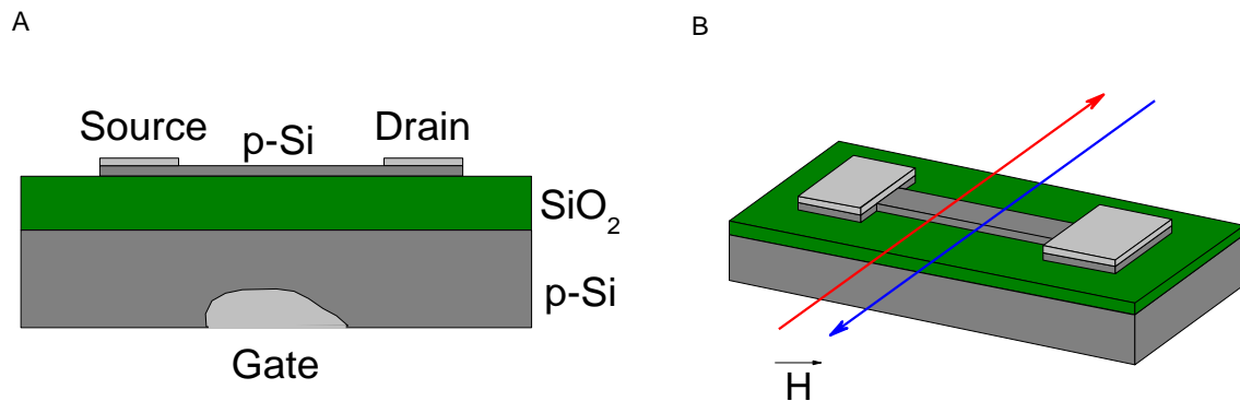
Figure 1(a, b). (a) The SiNWFET structure scheme, (b) experimental geometry.
