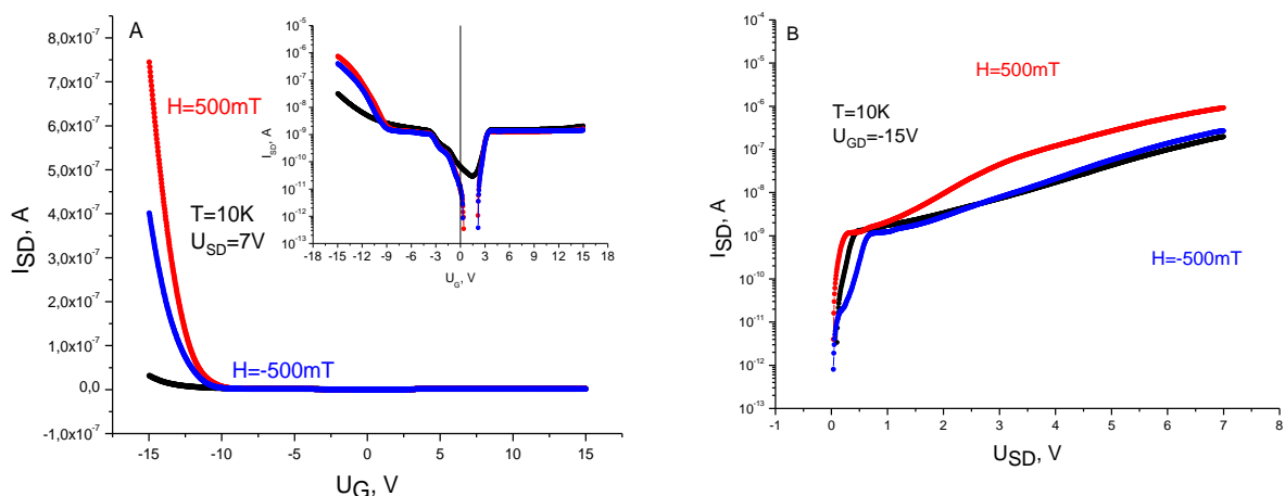
Figure 2(a, b). (a) The transfer characteristics of the structure with a channel width of 500 nm in a magnetic field of 500 mT of different polarity (the inset shows the same data plotted on a semilog scale), (b) VCC of the device.
