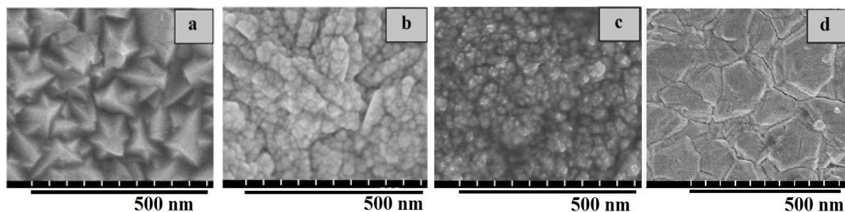
Figure 1. SEM images of the FeCo films surface prepared with different reducing agent: a – \text{Fe}/\text{Co} = 1.22 (sodium hypophosphite); b – \text{Fe}/\text{Co} = 0.5 series A; c – \text{Fe}/\text{Co} = 0.2 series C, d – \text{Fe}_{94}\text{Co}_6 series C.
