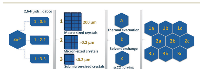
Fig. 1 Schematic overview of the DUT-8(Zn) samples synthesized using different precursor concentrations and desolvated under varying activation conditions.
