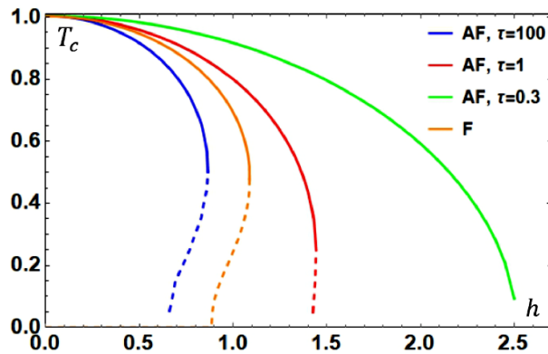
Figure 3. Critical temperature of the AF/S bilayer as a function of the effective exchange field induced by the antiferromagnet in the superconductor for different values of the impurity scattering time \tau , which is measured in units of the inverse superconducting critical temperature of the bulk superconductor.
