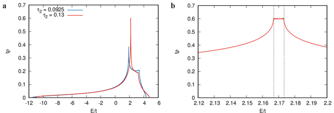
Figure 1. a DoES for FCC lattice at \tau_1 = -0.13 , \tau_2 = 0.0925 и 0.13 in full energy interval; b this quantity in the vicinity of the peak \tau_2 = 0.13 .
