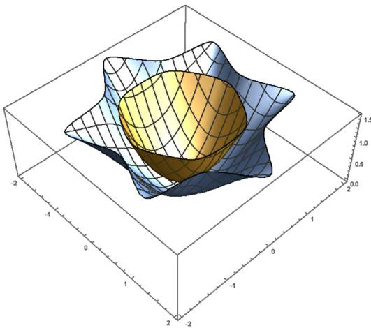
Figure 1. The lowest GaN/AlN 2DEG QWS dispersion with account for SOC.
