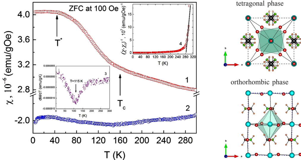
Figure 1. Temperature dependence of the magnetic susceptibility in \text{CH}_3\text{NH}_3\text{PbI}_3 single crystal. Curve 1 is obtained at the parallel orientation of the magnetic induction vector with respect to the (001) plane, curve 2 – at the perpendicular orientation of the magnetic induction vector with respect to the (001) plane, curve 3 is the derivative dM/dT , curve 4 is the inverse susceptibility with the Curie-Weiss fitting.
