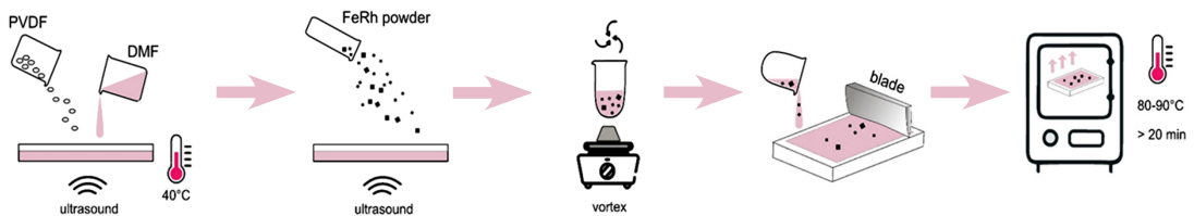
Figure 1. Fabrication scheme of 0-3 type PVDF based composite.
