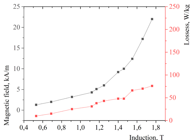
Figure 1. Electromagnetic characteristics of composite based on ABC100.30 powder.
