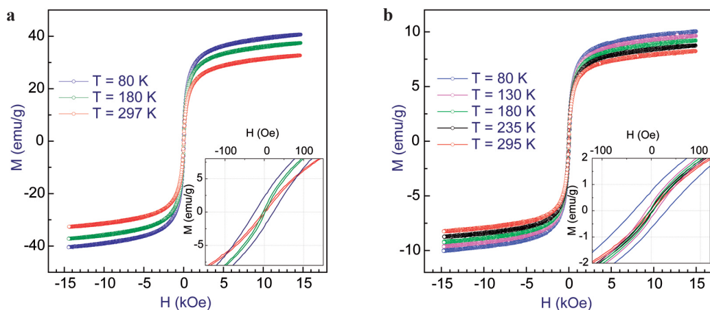
Figure 1. Hysteresis loops of magnetic nanoparticles. a \text{Fe}_3\text{O}_4:\text{SiO}_2 = 1:1.3 , b \text{Fe}_3\text{O}_4:\text{SiO}_2 = 1:4.5 .
