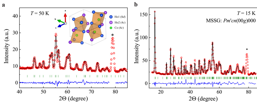
Figure 1. Neutron powder diffraction patterns for \text{Ho}_3\text{Co} measured in a paramagnetic state at T = 50 K (a) and below the Neel temperature at T = 15 K (b). The best fit result at T = 15 K provided by a model of the magnetic superspace group Pm'cn(00g)000 is shown as a solid line through the symbols.
