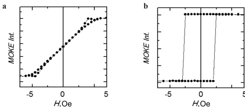
Figure 1. Hysteresis loops taken along the deposition field direction for the films of different compositions: a Fe 10 Ni 90 film (hard magnetization axis), b Fe 19 Ni 81 film (easy magnetization axis). Longitudinal magneto-optical Kerr effect.
