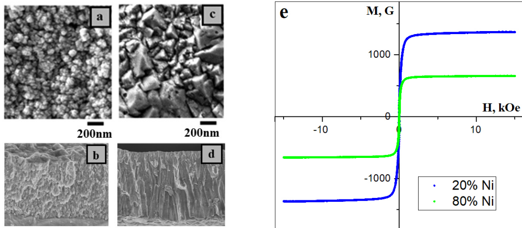
Figure 1. SEM images of the surface morphology and cross section of the FeNi-C films prepared with different reducing agent: arabinogalactan (a, b), sucrose (c, d). Hysteresis loops for FeNi-C films produced with different Ni content (e).
