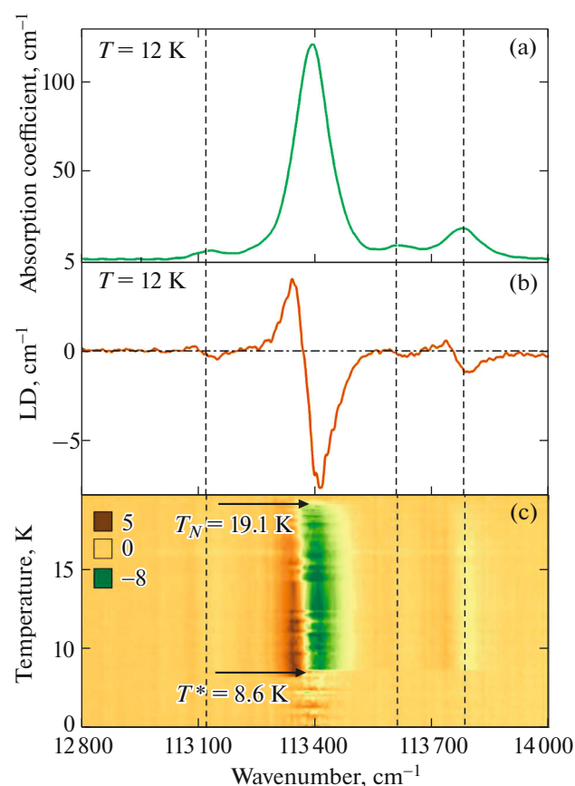
Fig. 3. Spectra of \text{Cu}_{0.9}\text{Ni}_{0.1}\text{B}_2\text{O}_4 crystal in the region of the first exciton ZPL \text{Cu}(4b) : absorption spectra at 12 K (a); LD spectra at 12 K (b); LD spectra presented as a color intensity map in the wavenumber—temperature axes (c).
