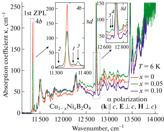
Fig. 1. Absorption spectra of \text{Cu}_{1-x}\text{Ni}_x\text{B}_2\text{O}_4 : x = 0, 0.05, 0.1 in a -polarization ( \mathbf{k} \parallel c, \mathbf{E} \perp c, \mathbf{H} \perp c ) at a temperature of 6 K. The arrows show the satellites of the first ZPL in \text{Cu}_{1-x}\text{Ni}_x\text{B}_2\text{O}_4 spectra associated with the distortion of the crystal lattice due to the inclusion of \text{Ni}^{2+} ion.
