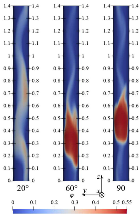
Fig. 1. Distribution of volume concentration at channel bottom surface. Inclination angle \alpha = 20^\circ, 60^\circ, 90^\circ
