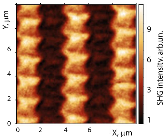
Figure 1. SHG microscopy image ( \lambda_0=850 nm) of the interface LuBiFeO/GGG interface layer.
