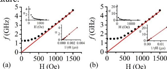
Figure 1. Dependence of the FMR resonant frequency on the external field H of the NiFe 2 O 4 nanoparticles (a) and particles coated with PVA (b).
