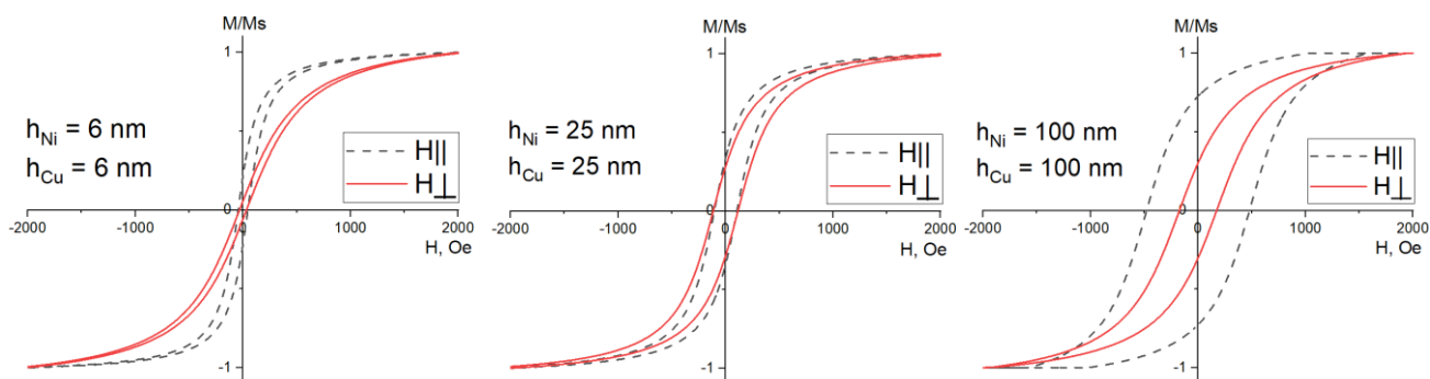
Fig.1. The hysteresis loops for layered nanowires with 30 nm diameter and various layer AR
