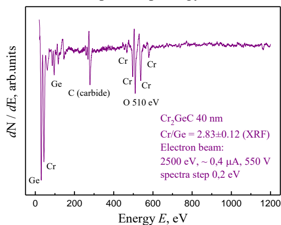
Figure 1. Auger electron spectra of Cr_2GeC MAX phase on MgO with a shift of peaks
