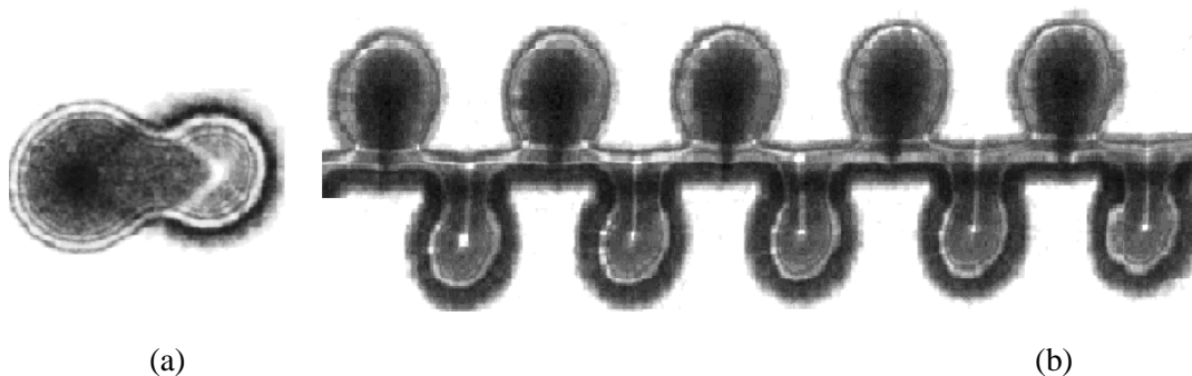
Figure 1. LTEM image of overlapping Permalloy disks (a) and system of disks-nanowire (b). The lateral dimensions of the discs are 1 micron.
