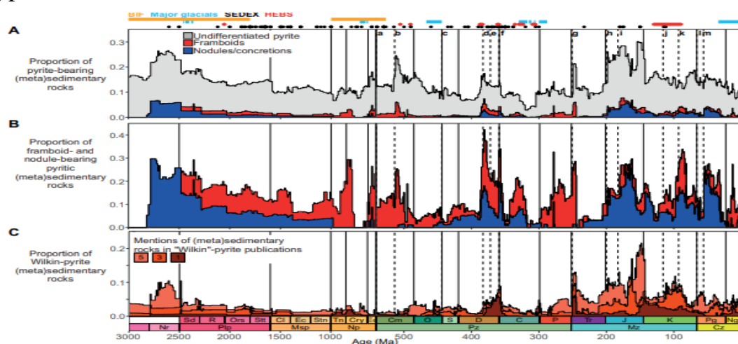
Figure. Stacked abundances of pyrite-bearing sedimentary and metasedimentary rocks through geological time. (A and B) Pyrite framboid– and nodule-bearing rocks expressed as proportions of all (meta)sedimentary rocks (A) and all pyrite-bearing (meta)sedimentary rocks (B).
