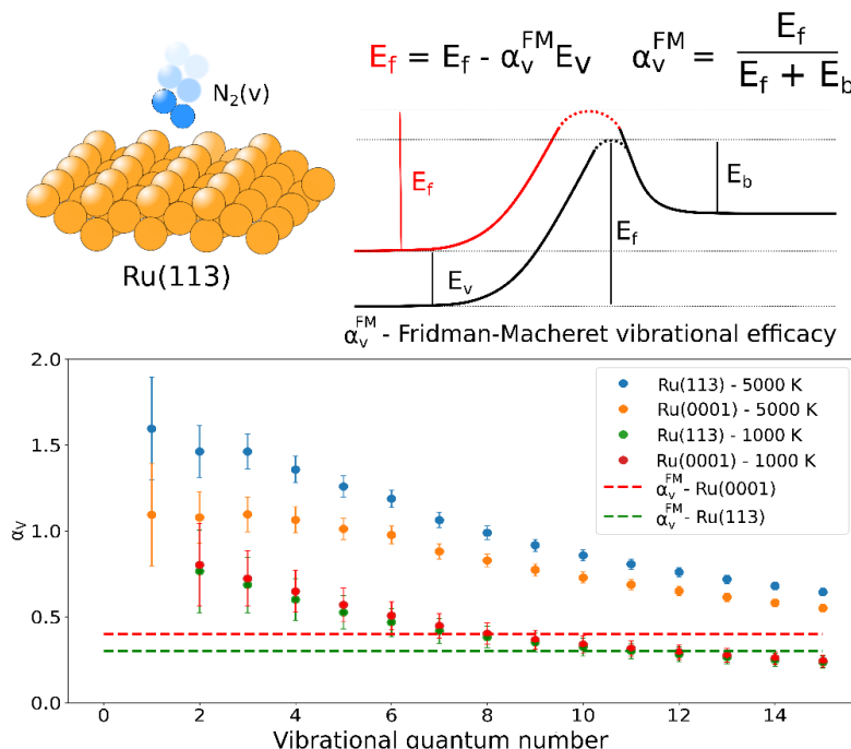
Fig. 1: The dependence of \alpha -v on vibrational quantum number for T = 1000, 5000 K for Ru(0001) and Ru(113)
