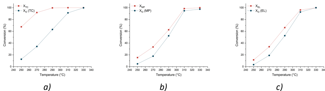
Fig. 1. a) Tricaprylin (TG), b) methyl palmitate (FAME), c) ethyl laurate conversion and O conversion vs temperature over Ni_2P/Al_2O_3 . P = 3 \text{ MPa} , LHSV = 90 \text{ h}^{-1} , H_2/feed = 600 \text{ Ncm}^3/\text{cm}^3
