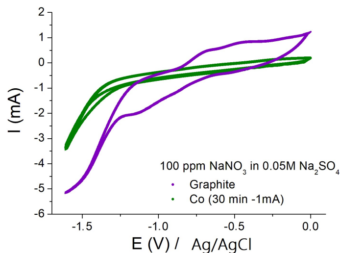
Fig. 2. Typical CV curves illustrating significant progress in ammonia synthesis at the reaction potential E=(-1.3)-(-1.4) V vs Ag/AgCl for graphite substrate and deposited catalyst (nanocobalt, 30 min deposition) in a pH-neutral nitrate-sulfate electrolyte.
