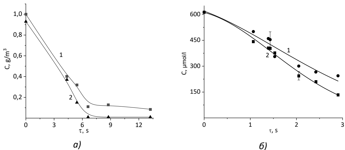
Fig. 1. Changes in the content of 2,4-DCP in vapor-gas mixtures (a) and aqueous solutions (b) in plasma (1) and plasma-catalytic (2) processes.
