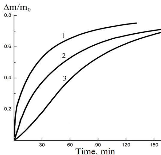
Fig. 2. Kinetic curves of relative mass reduction during the thermal degradation of the original polycarbonate (2); non-irradiated (1) and irradiated (3) polycarbonate films containing 0.01 wt. % TiO 2 nanoparticles; T=420°C.
