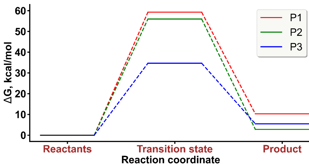
Fig. 1. Energy profile of the reaction of 1,2-insertion of propene at the Zr-C bond of various \text{Cp}_2\text{ZrMeCl} -MAO complexes
