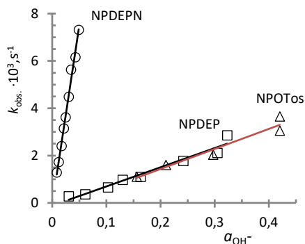
Fig.1. First order rate constants k_{obs} , s^{-1} vs hydroxide concentration a_{OH^-} for base catalysed hydrolysis of some esters; water, 25°C
