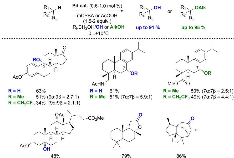
Fig. 2. Oxidative functionalization of complex substrates of natural origin.
