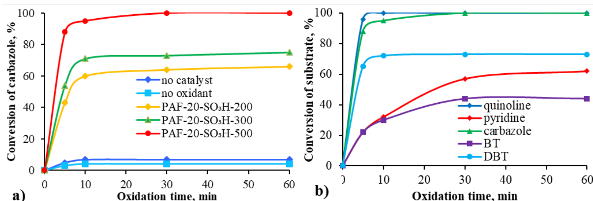
Fig. 2. A. Catalysts activity test cycles (oxidation conditions: 2,0 wt% of catalyst, H 2 O 2 :N molar ratio of 4:1, T 80°C). B. Oxidation of various substrates (oxidation conditions: 2,0 wt% of catalyst PAF-20-SO 3 H-500, H 2 O 2 :N molar ratio of 4:1, T 80°C).
