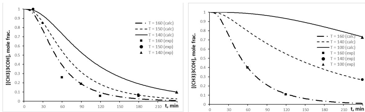
Fig. 2. Change in tert-butanol concentration in the presence of HY and CuBr 2 /HY
