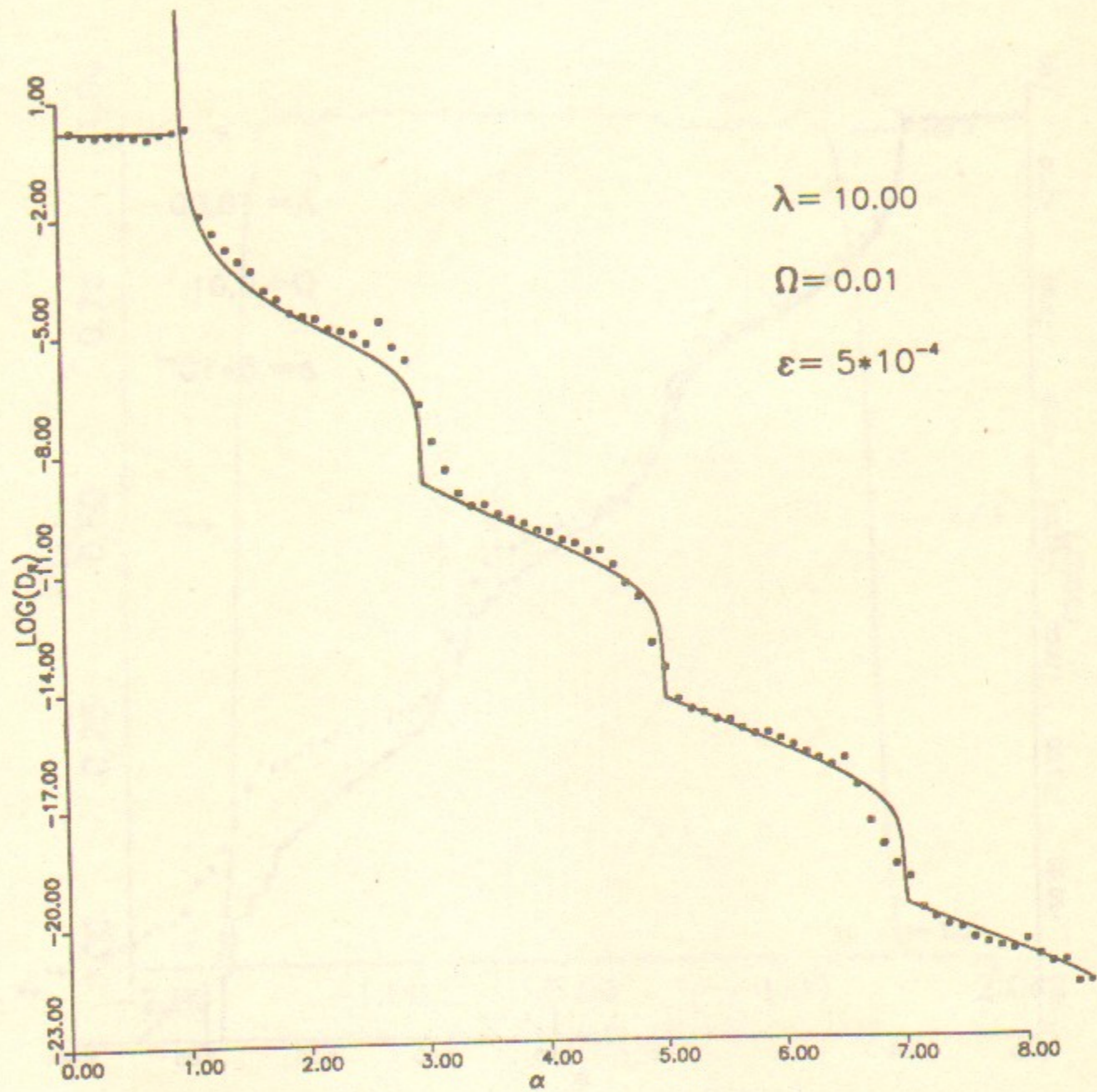
Fig.5. Scaled diffusion coefficient (unmodulated driving resonance).
