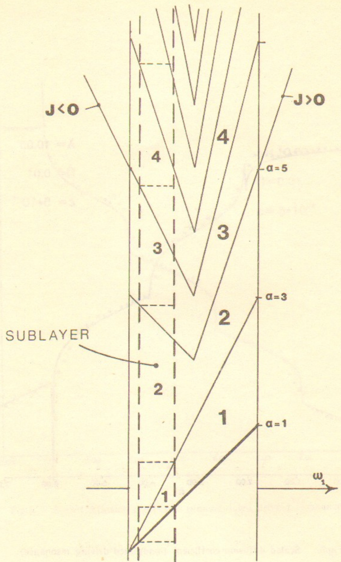
Fig.7. Sublayer diffusion: map of interaction regions ( q=1 ).
