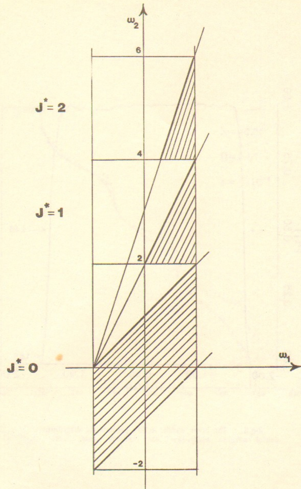
Fig. 2. Geometrical structure of a modulational layer (modulated driving resonance, q=1 ).
