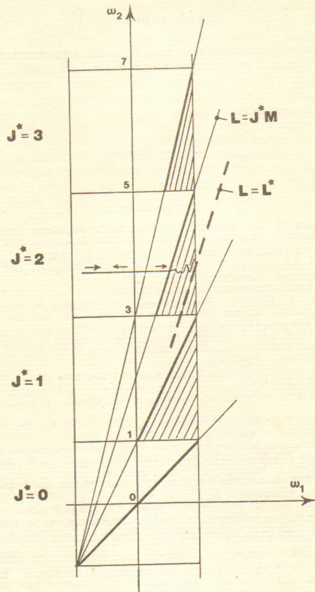
Fig. 1. Geometrical structure of a modulational layer (unmodulated driving resonance, q=1 ).
