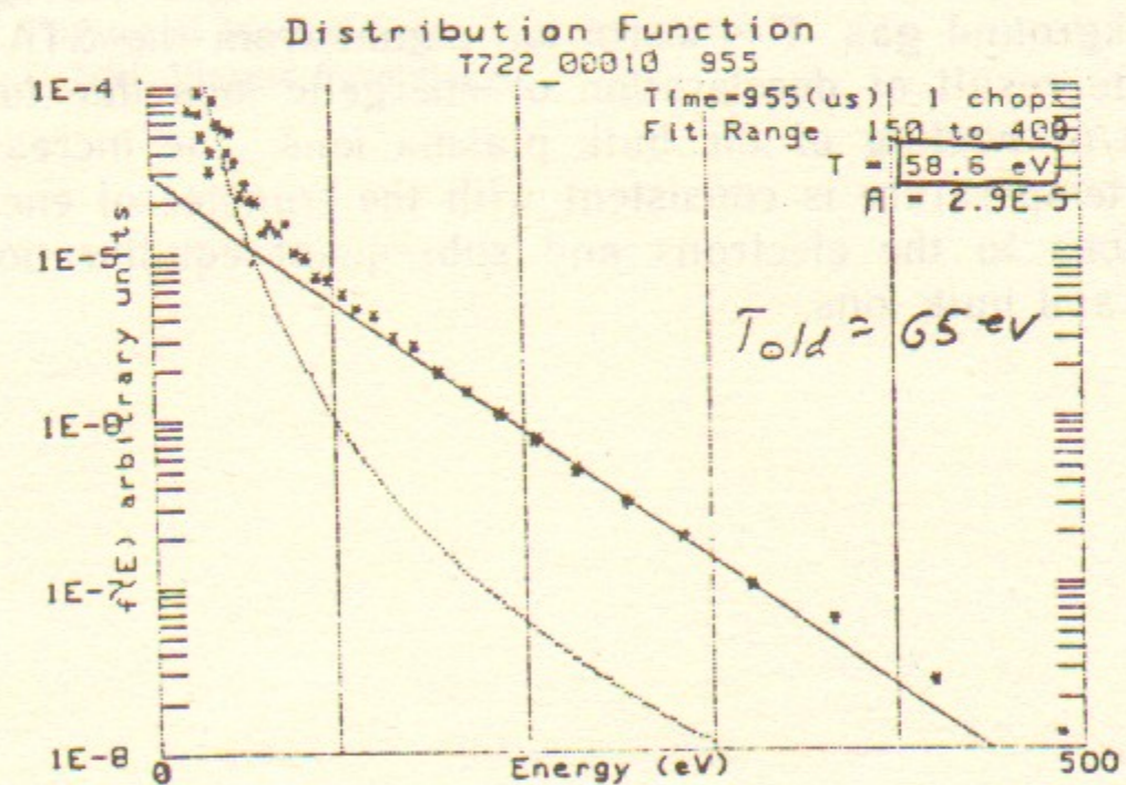
Fig. 24. The effect of neutral attenuation on the determination of the ion temperature.
