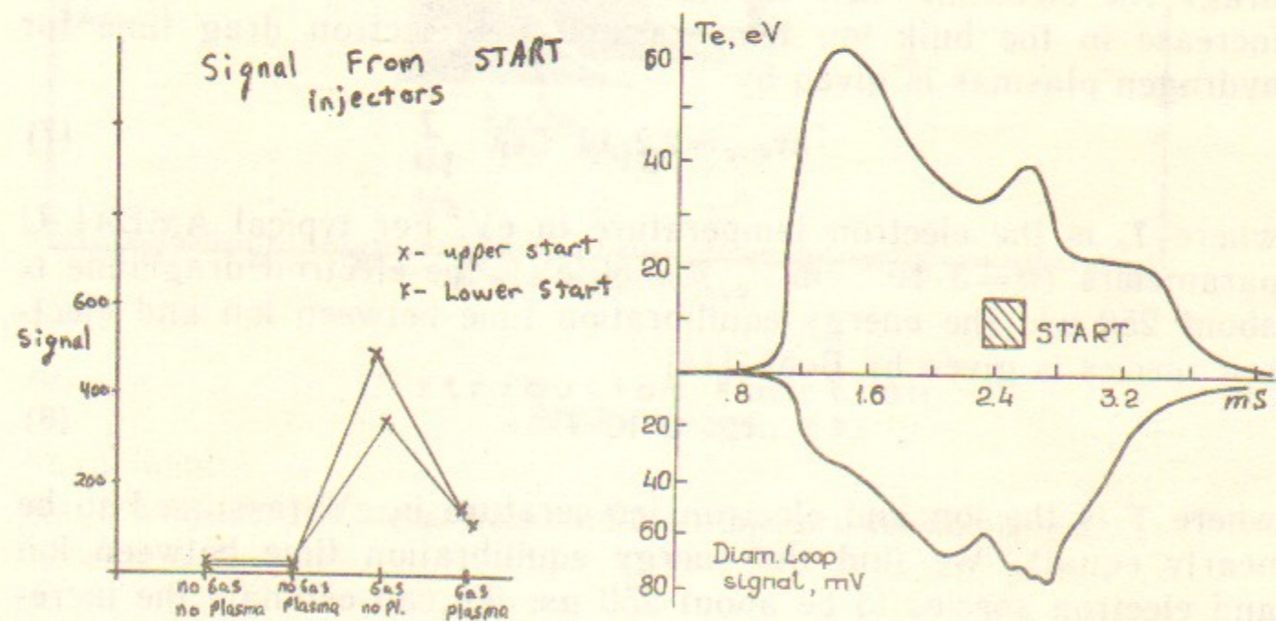
Fig. 21. Signal from the START injectors under various operating conditions.
